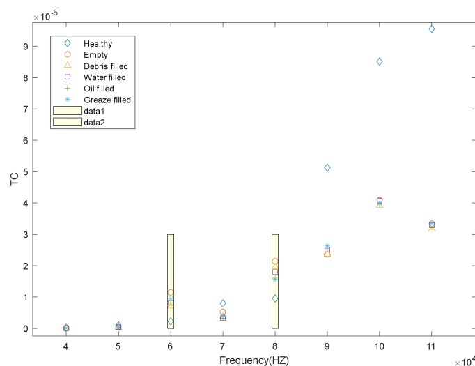
Figure 27. Different case transmission coefficients vs. frequency.
