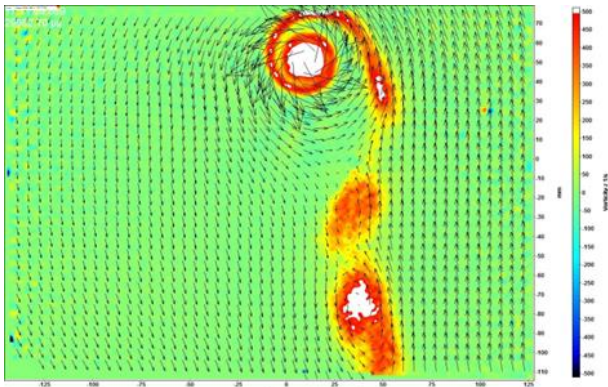
Fig 9: Time-averaged vorticity ( \zeta , /s) distribution in a plane orthogonal to the free stream 0.303b downstream of the wing tip, zero outboard aileron deflection.
