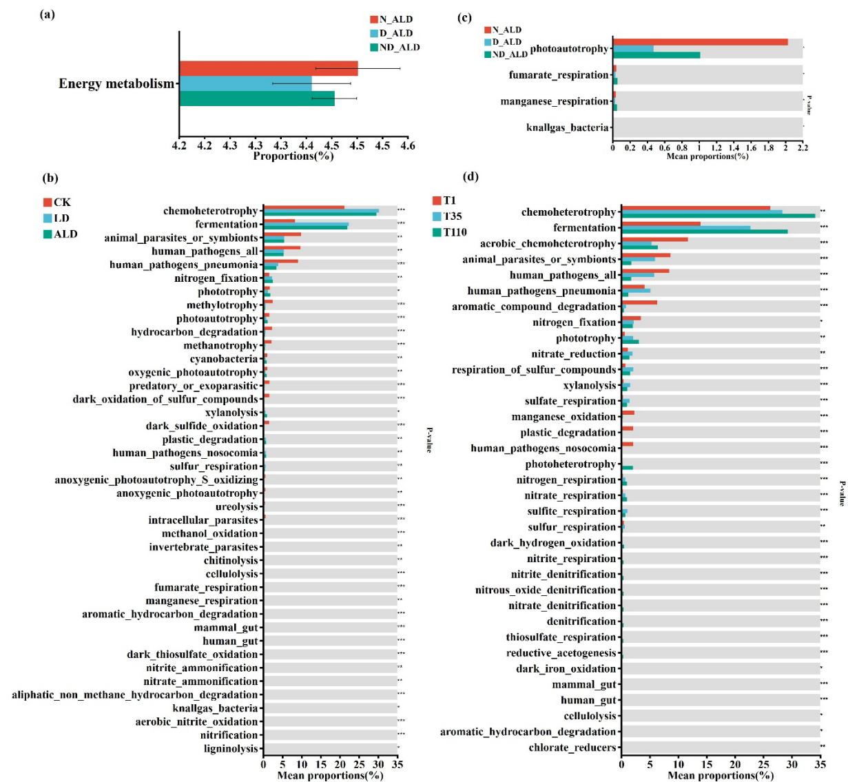
Fig.S9 Bacterial functional pathways showing significant differences at Level 2 (a) by PICRUST2 analysis based on the KEGG database in the N-ALD, D-ALD and ND-ALD group and ecologically relevant functional groups of bacteria showing significant differences via FAPROTAX analysis (b-d) (Control group (CK), litter decomposition group (LD), antibiotic-litter decomposition group (ALD), norfloxacin-litter decomposition group (N-ALD), doxycycline-litter decomposition group (D-ALD), a combination of both antibiotics-litter decomposition group (ND-ALD)). * P < 0.05 ; ** P < 0.01 ; *** P < 0.001 )
