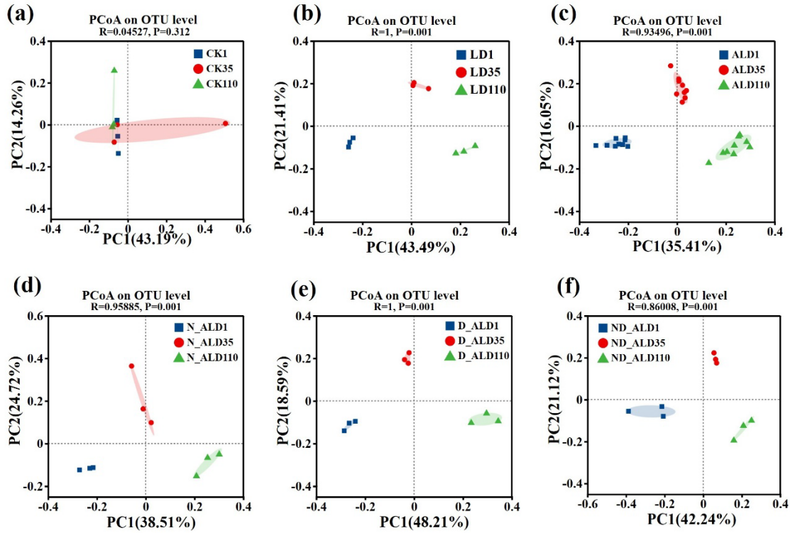
Fig. S5 Principal co-ordinate analysis (PCoA) of the bacterial community structure of CK (a), LD (b), ALD (c), N-ALD (d), D-ALD (e) and ND-ALD (f) group on day 1, 35 and 110 of litter decomposition. (Control group (CK), litter decomposition group (LD), antibiotic-litter decomposition group (ALD), norfloxacin-litter decomposition group (N-ALD), doxycycline-litter decomposition group (D-ALD), a combination of both antibiotics-litter decomposition group (ND-ALD))
