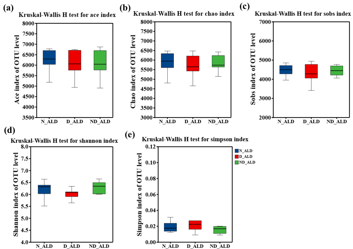
Fig. S3 Kruskal-Wallis H test bar plot of alpha diversity indices of N-ALD, D-ALD and ND-ALD group in sediment. (Norfloxacin-litter decomposition group (N-ALD), doxycycline-litter decomposition group (D-ALD), a combination of both antibiotics-litter decomposition group (ND-ALD)). * and ** indicate significant differences ( P < 0.05 and P < 0.01 )
