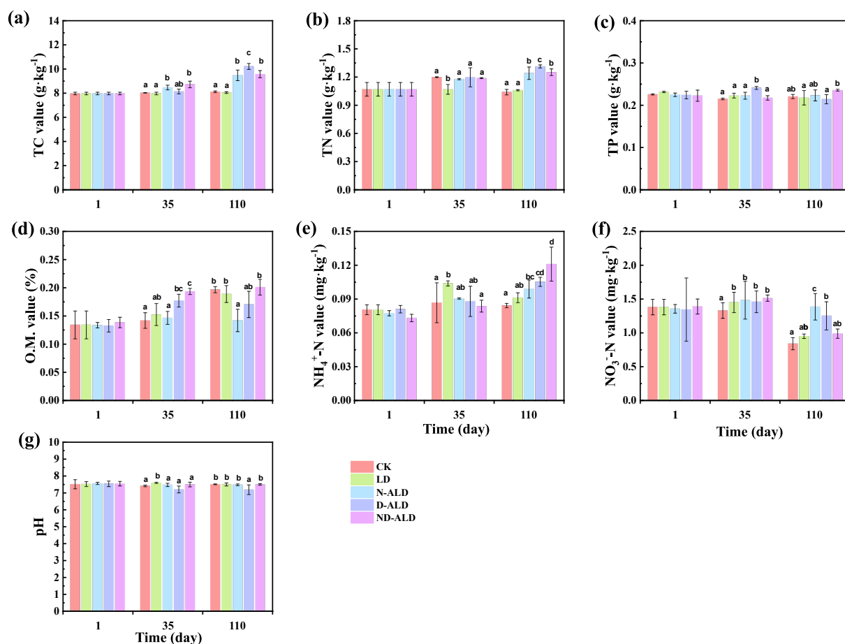
Fig. S2 Physicochemical parameters (TC (a), TN (b), TP (c), O.M. (d), \text{NH}_4^+\text{-N} (e), \text{NO}_3^-\text{-N} (f) and pH (g)) of sediment during the litter decomposition processing. (Control group (CK), litter decomposition group (LD), antibiotic-litter decomposition group (ALD), norfloxacin-litter decomposition group (N-ALD), doxycycline-litter decomposition group (D-ALD), a combination of both antibiotics-litter decomposition group (ND-ALD). Means with a common letter are significantly different ( P < 0.05 ))
