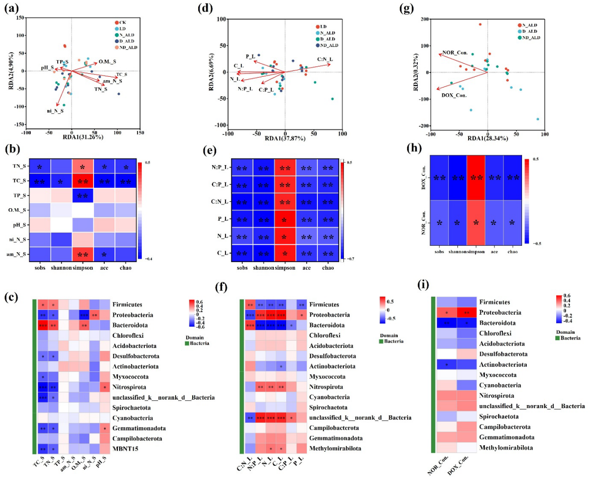
Fig S11 Correlation between sediment physicochemical properties (a-c), litter nutrient (d-f) and antibiotics concentration (g-i) on sediment community structure, microbial alpha diversity indices and phylum species. ((Control group (CK), litter decomposition group (LD), antibiotic-litter decomposition group (ALD), norfloxacin-litter decomposition group (N-ALD), doxycycline-litter decomposition group (D-ALD), a combination of both antibiotics-litter decomposition group (ND-ALD)). * P < 0.05 ; ** P < 0.01 ; *** P < 0.001 )
