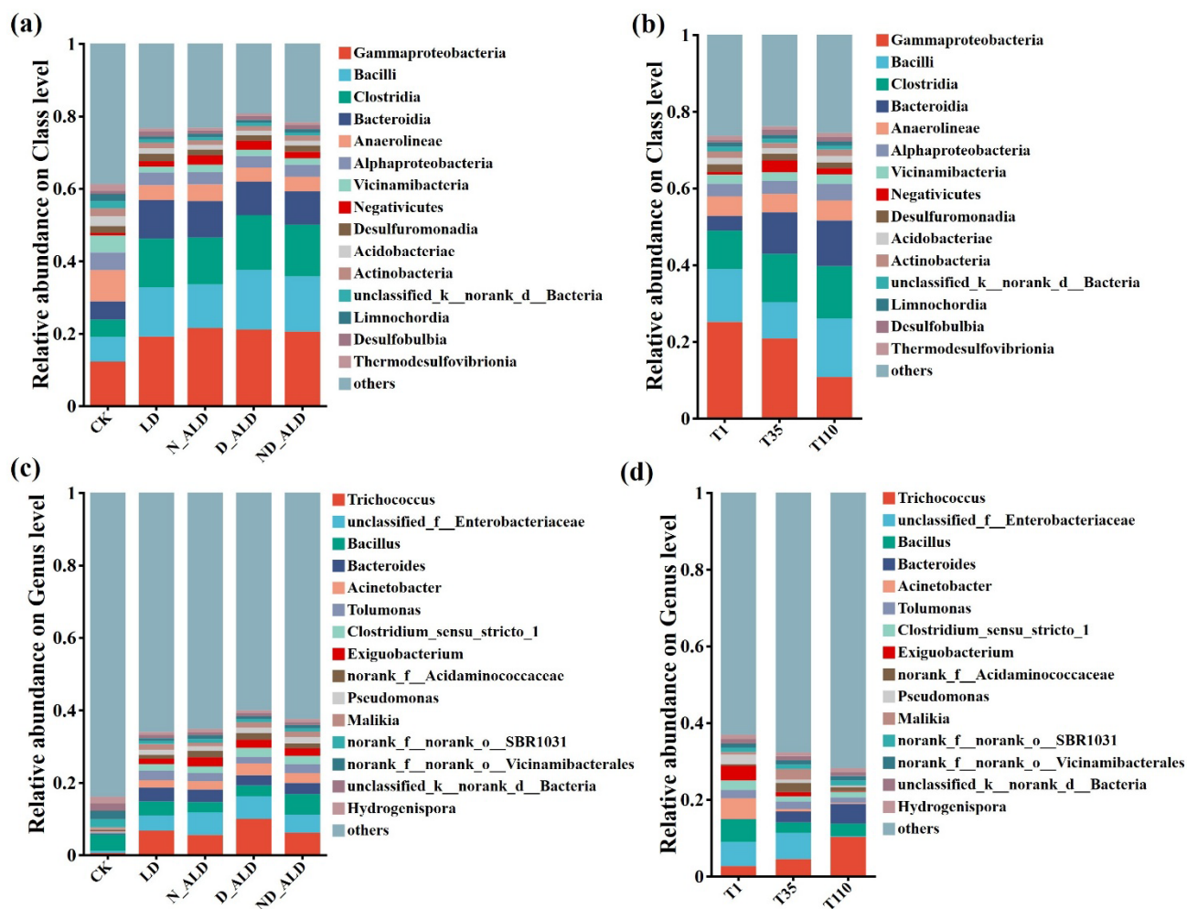
Fig.S7 The relative abundance of bacterial communities at Class (a-b) and genus (c-d) level. (Control group (CK), litter decomposition group (LD), antibiotic-litter decomposition group (ALD), norfloxacin-litter decomposition group (N-ALD), doxycycline-litter decomposition group (D-ALD), a combination of both antibiotics-litter decomposition group (ND-ALD))
