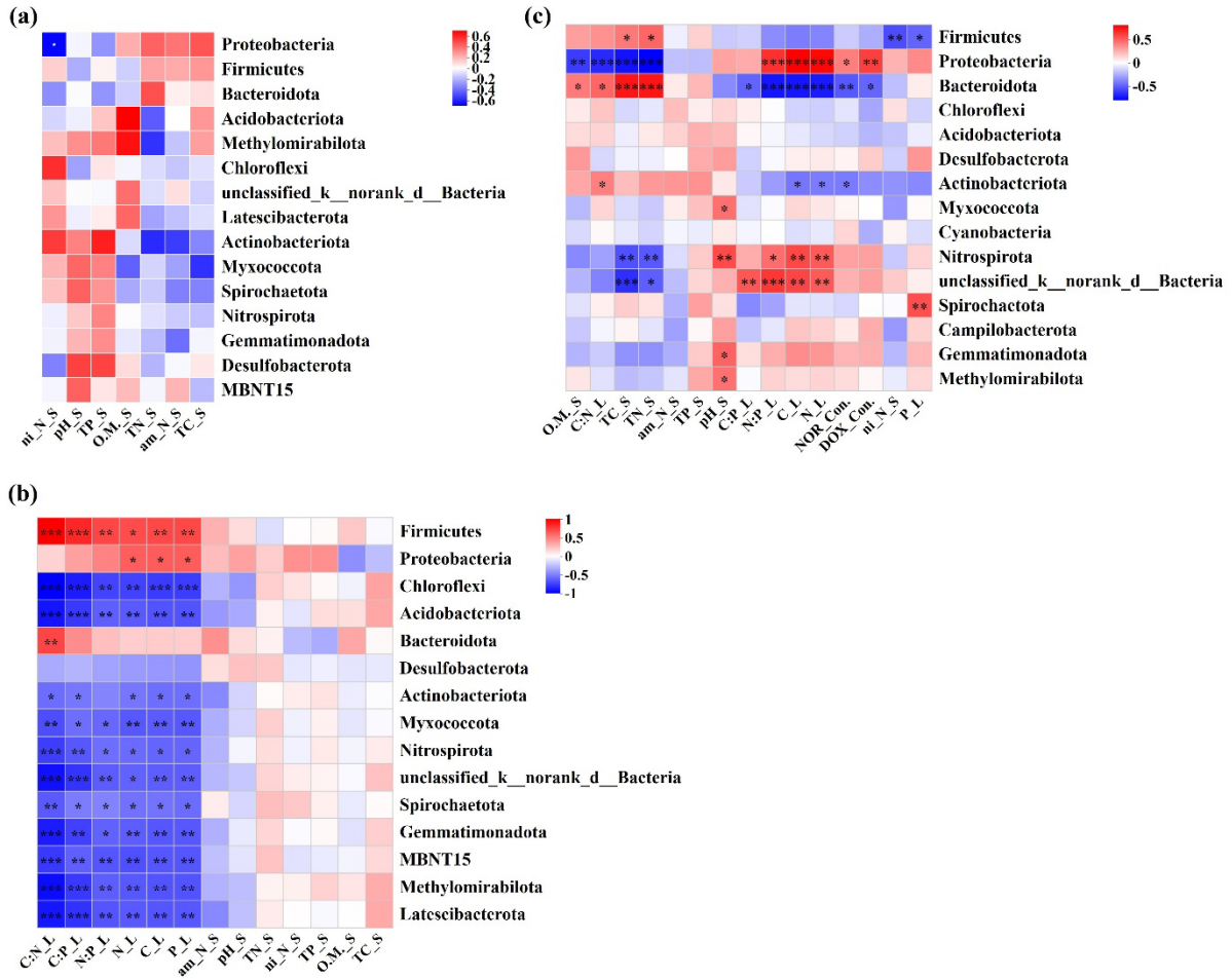
Fig S10 Spearman correlation heatmap of Phylum species with litters nutrients and the physicochemical parameters of sediment in the CK (a), LD (b) and ALD (c) groups. (Control group (CK), litter decomposition group (LD), and antibiotic-litter decomposition group (ALD)). * P < 0.05 ; ** P < 0.01 ; *** P < 0.001 )
