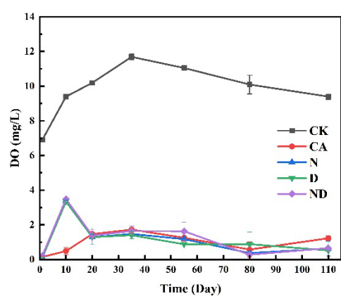
Fig S12 Physicochemical indicators DO of overlying water. (Control group (CK), litter decomposition group (LD), antibiotic-litter decomposition group (ALD), norfloxacin-litter decomposition group (N-ALD), doxycycline-litter decomposition group (D-ALD), a combination of both antibiotics-litter decomposition group (ND-ALD))
