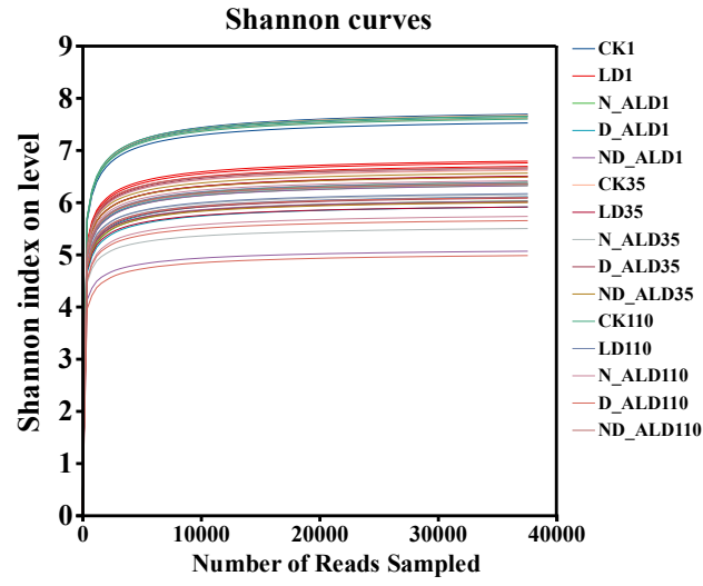
Fig. S1 Shannon curves of bacterial microorganisms in freshwater sediment. (Control group (CK), litter decomposition group (LD), antibiotic-litter decomposition group (ALD), norfloxacin-litter decomposition group (N-ALD), doxycycline-litter decomposition group (D-ALD), a combination of both antibiotics-litter decomposition group (ND-ALD). * and ** indicate significant differences ( P<0.05 and P<0.01 ))
