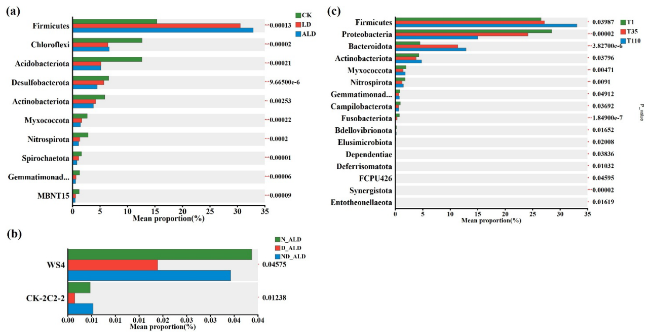
Fig.S8 Kruskal-wallis H test bar plot of community composition between CK, LD and ALD group (a), and N-ALD, D-ALD and ND-ALD group (b) and day 1, 35 and 110 (c) at phylum level (Control group (CK), litter decomposition group (LD), antibiotic-litter decomposition group (ALD), norfloxacin-litter decomposition group (N-ALD), doxycycline-litter decomposition group (D-ALD), a combination of both antibiotics-litter decomposition group (ND-ALD)). * P < 0.05 ; ** P < 0.01 ; *** P < 0.001 )
