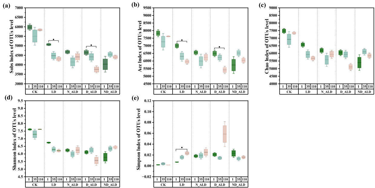
Fig. S4 Kruskal-Wallis H test bar plot of alpha diversity indices of CK, LD, N-ALD, D-ALD and ND-ALD group 1, 35 and 110 of litter decomposition. (Control group (CK), litter decomposition group (LD), antibiotic-litter decomposition group (ALD), norfloxacin-litter decomposition group (N-ALD), doxycycline-litter decomposition group (D-ALD), a combination of both antibiotics-litter decomposition group (ND-ALD)).
