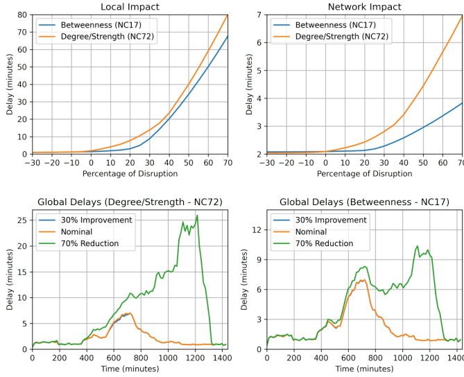
Fig. 4. Fragility and delay analysis of the AAM traffic network based on vertipoint disruptions.
