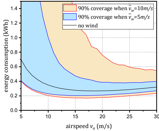
Fig. 4. Statistical distribution of energy consumption for a flight with the wind. In Monte Carlo simulations, the shape parameter of the wind Weibull distribution is set as 2.0.
