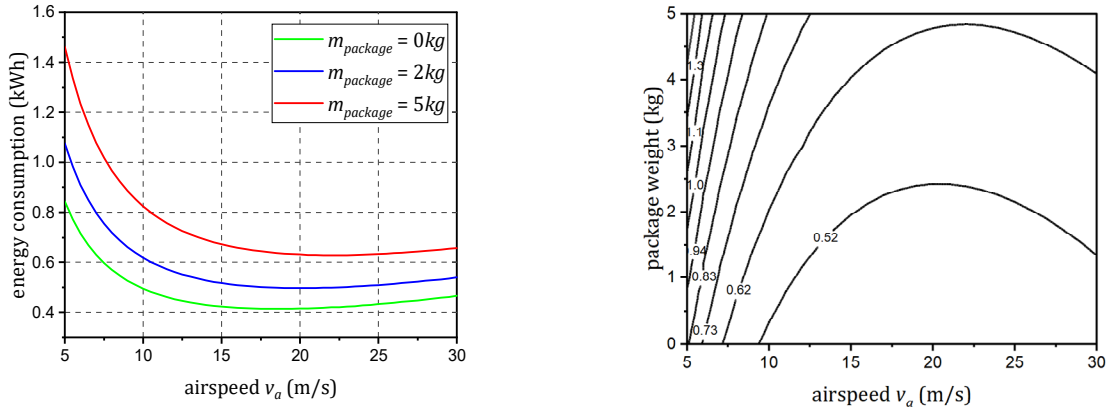
Fig. 3. Energy consumptions for a 10km flight with airspeed and package weight varying. In the first figure, three cases are considered with package weight 0 \text{ kg} , 2 \text{ kg} , 5 \text{ kg} respectively. In the second figure, a contour map of energy consumption is depicted with regard to airspeed and package weight. In simulations, no wind is considered, altitude for level flight h = 10 \text{ m} , hovering time T_{\text{hovering}} = 10 \text{ s} , and vertical speed is assumed as a constant v_v = 10 \text{ m/s} .
