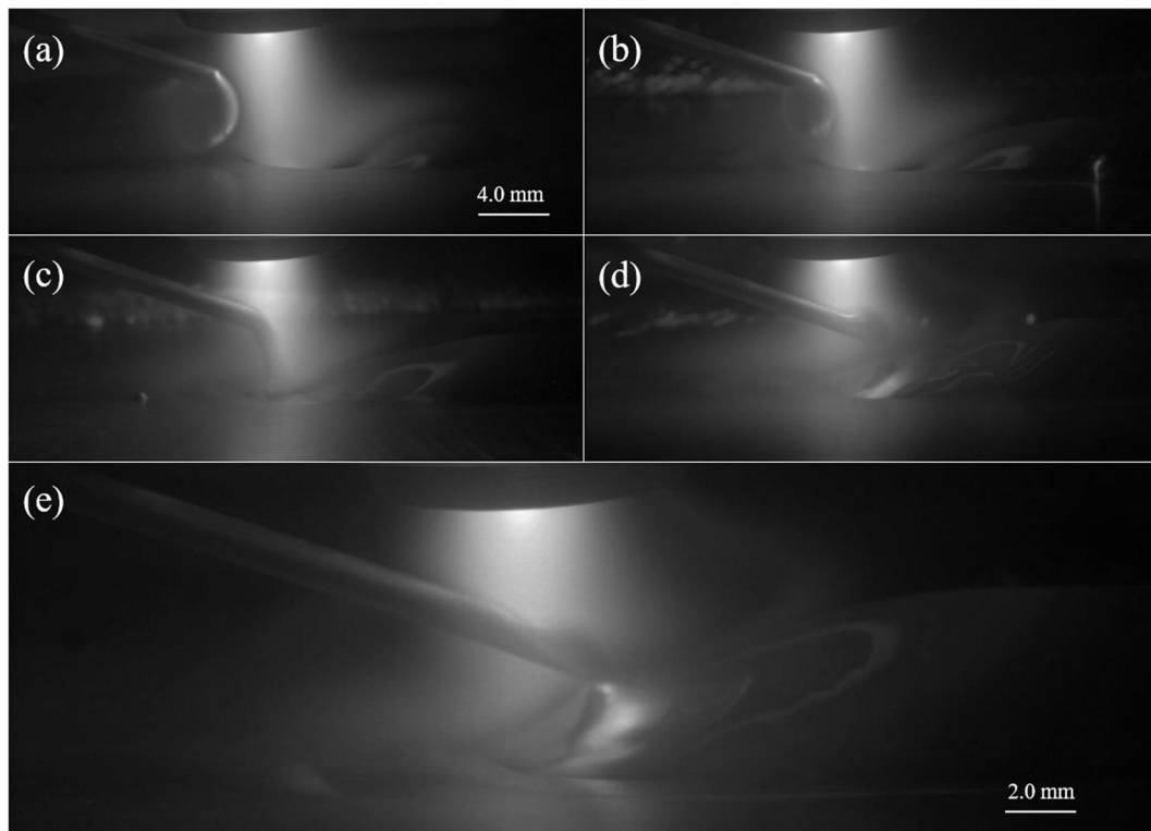
Fig. 10. Metal transfer images with different WFSs captured by a process camera: (a) 1 m/min; (b) 2 m/min; (c) 3 m/min; (d) 4 m/min; (e) 5 m/min.
