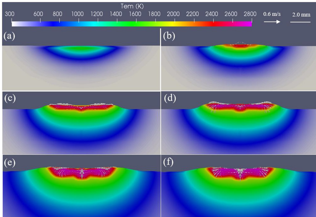
Fig. 7. Evolution of fluid flow in melt pool coupled the metal transfer dynamics with the WFS of 3 m/min at a transverse slice with 1.2 mm behind the arc centre: (a) 0.1186 s; (b) 0.2146 s; (c) 0.5746 s; (d) 0.6706 s; (e) 3.3106 s; (f) 3.3826 s.
