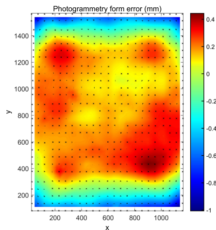
Figure 15. Photogrammetry form error map.
