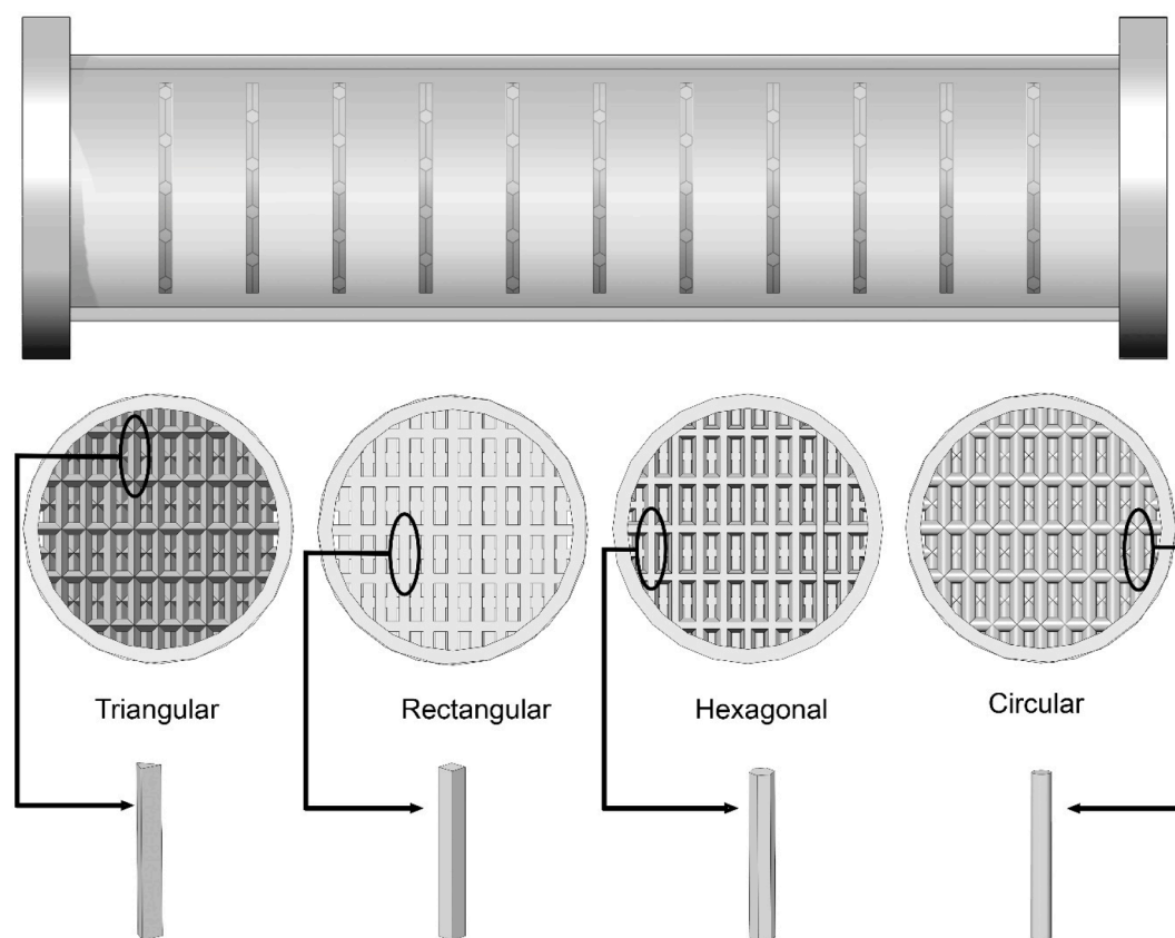
Fig 2. The schematic of catalyst monolith loaded with different catalytic monolith used to load the reactor for catalytic combustion of methane and hydrogen fuel.
