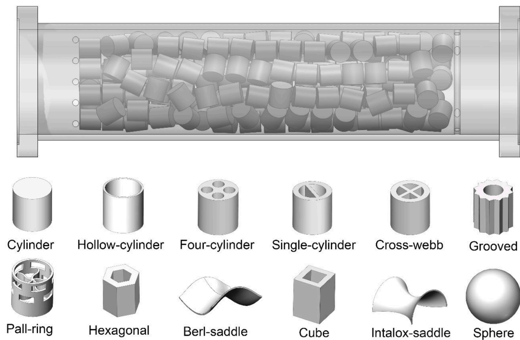
Fig 1. Schematic of the packed bed catalytic combustor and different packing loads for the analysis of the combustion of methane and hydrogen fuel.
