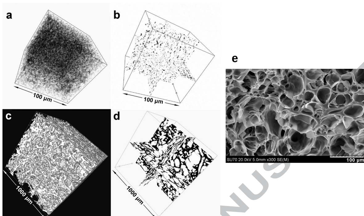
Figure 8: 3D degradation pattern in cured nanocomposite adhesive (1.0wt% \text{Fe}_3\text{O}_4 nanoparticles in epoxy resin); (a-b) before and (c-d) after microwave 3min exposure at 100 W, 2.45 GHz, (e) the FESEM magnified image of (c-d) [86]
