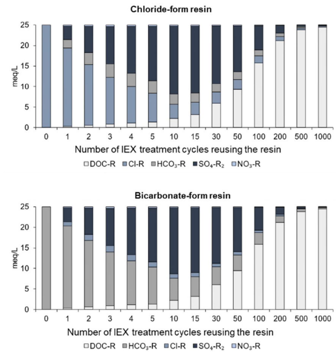
Figure 4. Modelled composition of the chloride- and bicarbonate-form resin loading over 1000 IEX treatment cycles
