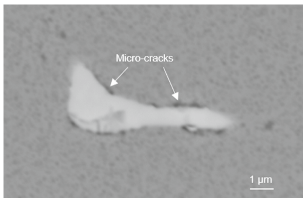
Fig. 7 Refractory metal carbide phase within IN6203DS superalloy showing micro-cracking at interface with the matrix
