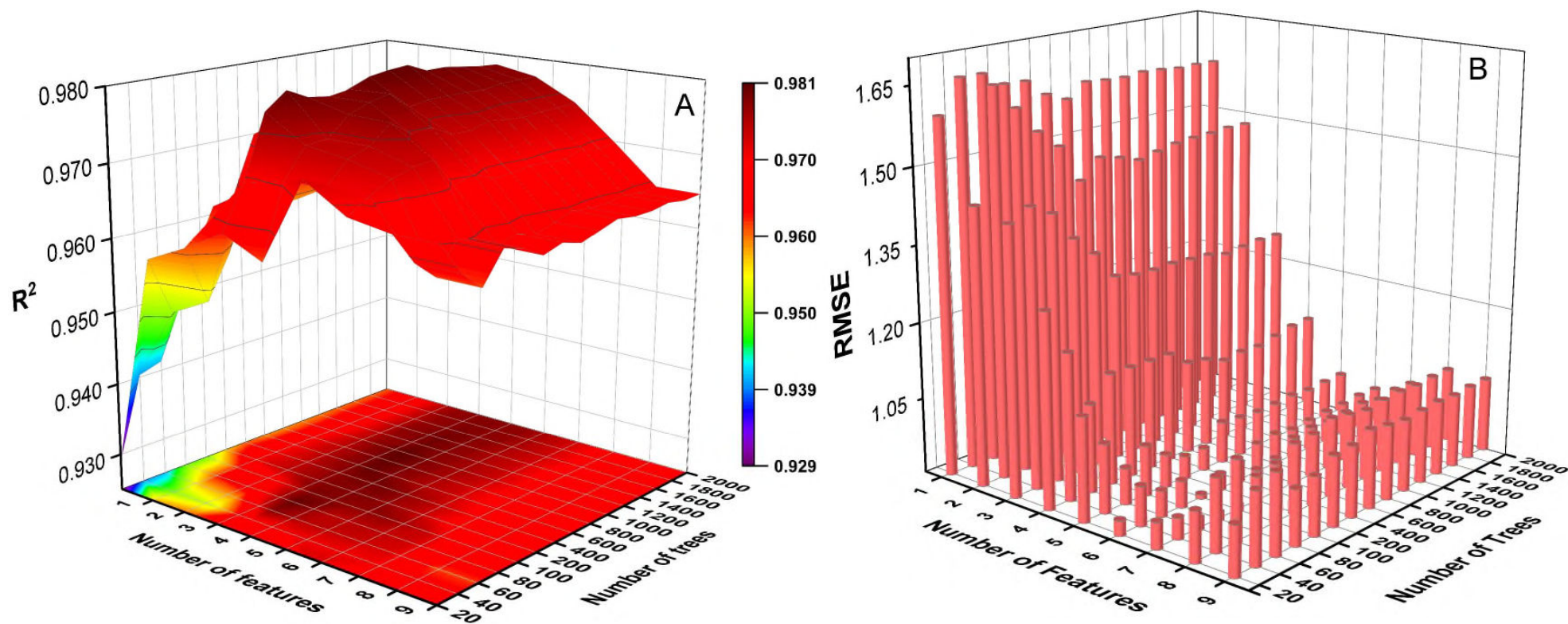
Fig. 2 Variance of R^2 and RMSE with the RF model parameters (optimal value: number of features = 6, number of trees = 100)
