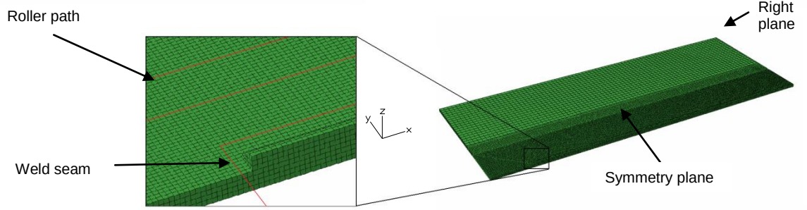
Figure 3: Mesh used in the analysis
