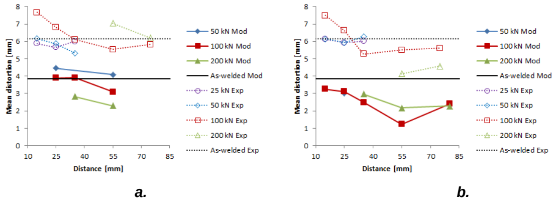
Figure 7: Mean distortion after PWR. a. Rolling on the top surface and b. bottom surface.
