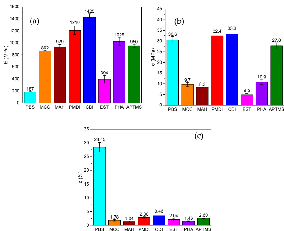
Figure 6. Tensile properties of PBS/MCC composites: (a) Elastic modulus E , (b) strength \sigma , and (c) strain \varepsilon .
