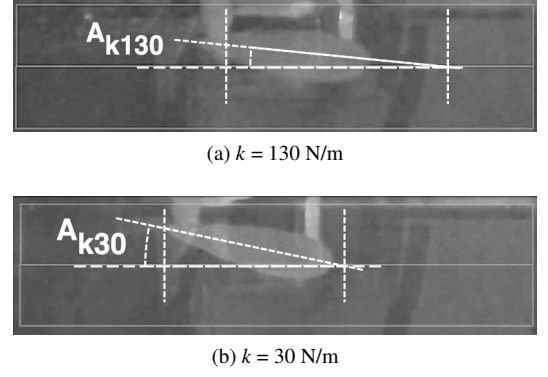
FIG. 6. Hydrofoil pose and flapping angle for (a) k = 130 N/m; (b) 30 N/m
