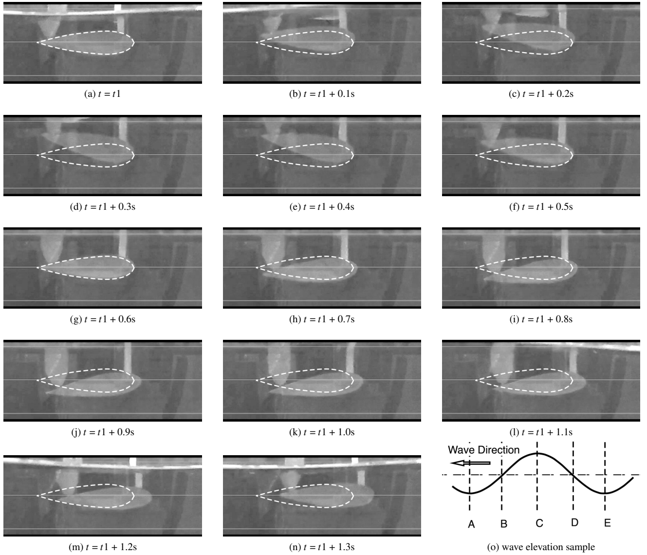
FIG. 7. (a)-(n): A complete cycle of hydrofoil underwater motion for k = 30 N/m with time interval 0.1 s; (o) wave elevation sample
