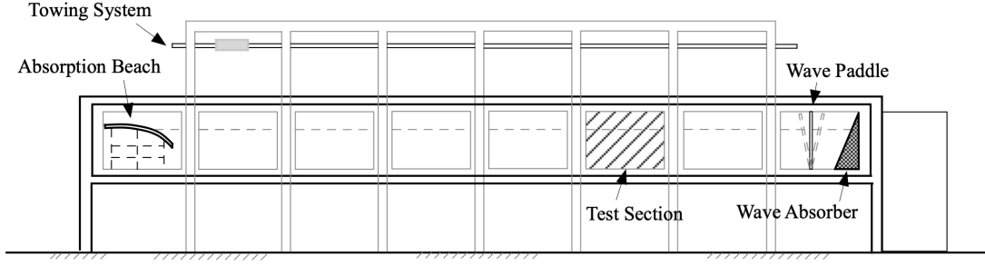
FIG. 2. Schematic sketch of the wave tank at Cranfield University
