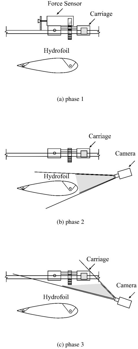
FIG. 4. Experimental arrangement for the pitch spring stiffness k = 130 N/m and 30 N/m for different phases: (a) phase 1; (b) phase 2; (c) phase 3
