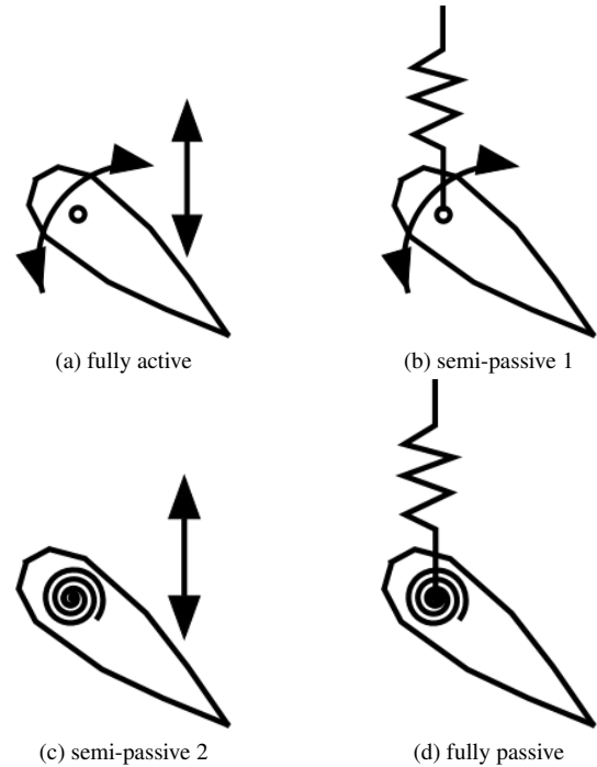
FIG. 1. Schematic sketch of (a) fully active motion; (b) (c) semi-passive motion and (d) fully passive motion
