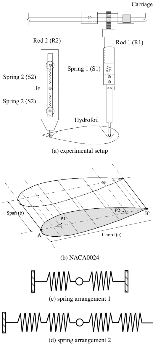
FIG. 3. Schematic sketch: (a) experimental setup; (b) NACA0024 foil; (c) spring arrangement 1; (d) spring arrangement 2
