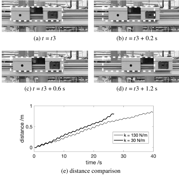
FIG. 9. (a)-(d): Film captures of moving carriage for k = 30 N/m at t = t_3 , t_3 + 0.2 s, t_3 + 0.6 s, t_3 + 1.2 s; (e) displacement of carriage against time for k = 130 N/m and 30 N/m
