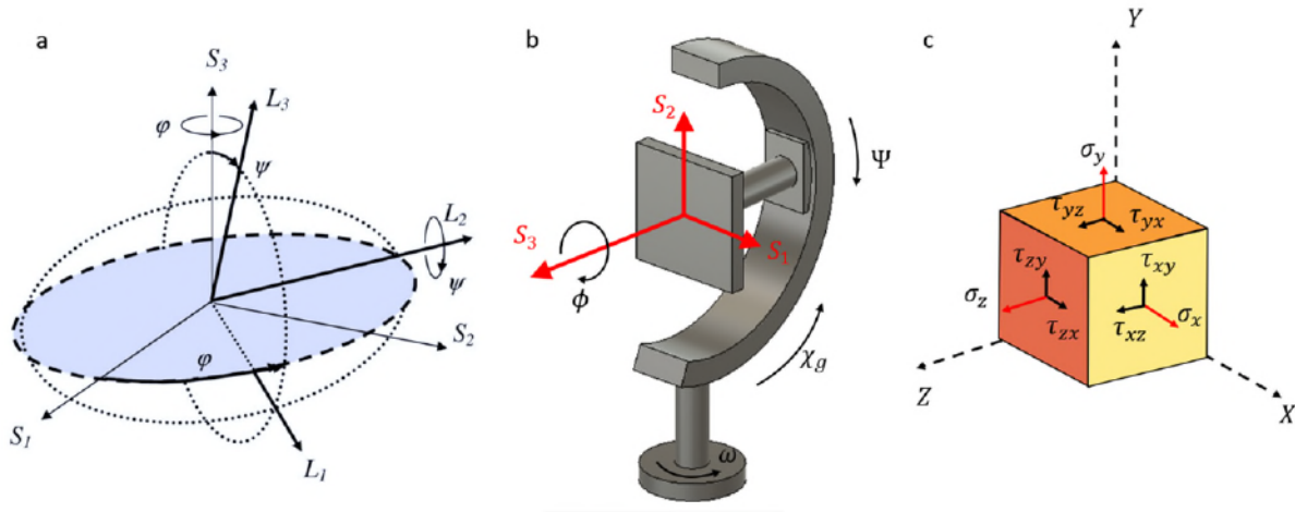
Fig 5: (a) Definition of, and relations between, the sample (S) and laboratory (L) reference frames (b) X-ray system configuration angles, and c general stress convention
