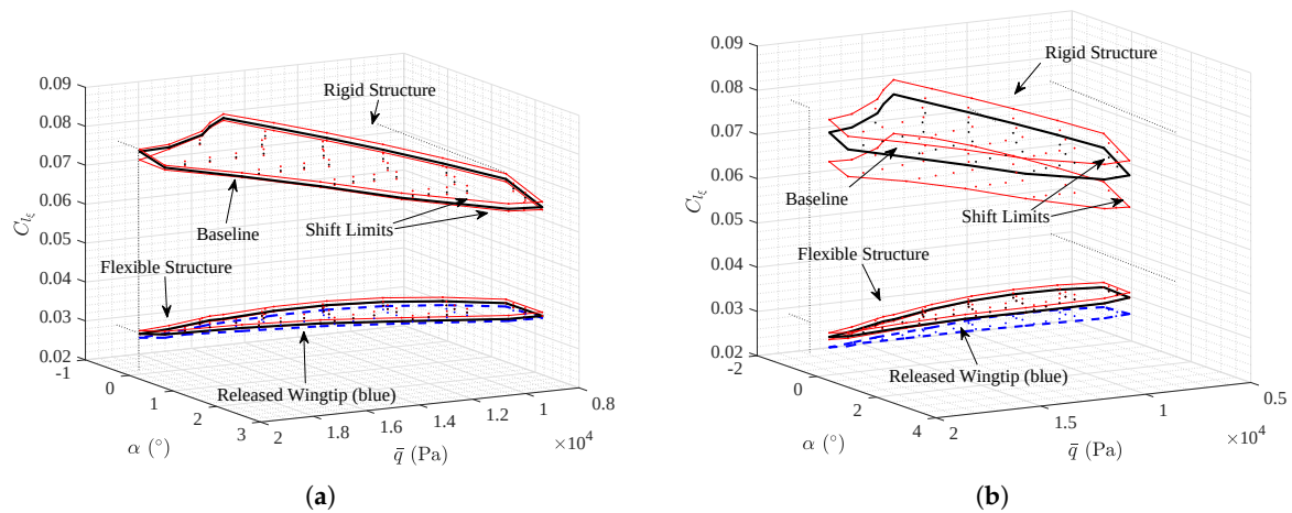
Figure 11. C_{l_\xi} variations against \bar{q} and \alpha_b : (a) 2.9 m (10% wing semispan) wingtip device; and (b) 5.8 m (20% wing semispan) wingtip device.
