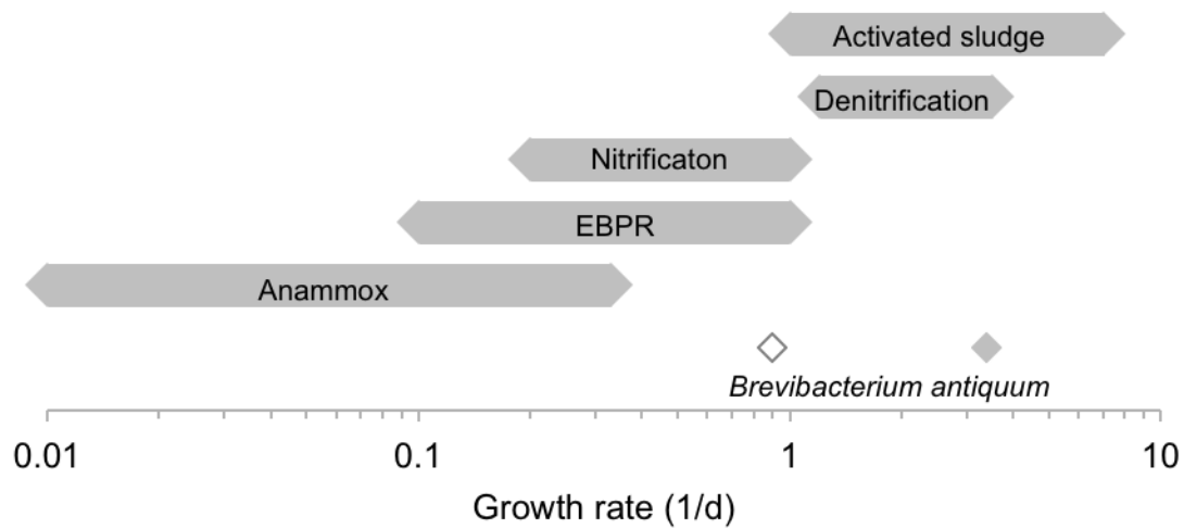
Figure 1 Comparison of the growth rates of B. antiquum in sludge dewatering liquors (◇, non-optimized; ◆, optimized with 3.0% w/v NaCl and 1124 mg COD/L as acetate) with the growth rate range of values found in published literature for heterotrophic bacteria in activated sludge systems, heterotrophic denitrifying bacteria, nitrification bacteria, enhanced biological phosphorus removal (EBPR) bacteria, and Anammox bacteria [23–25,27].
