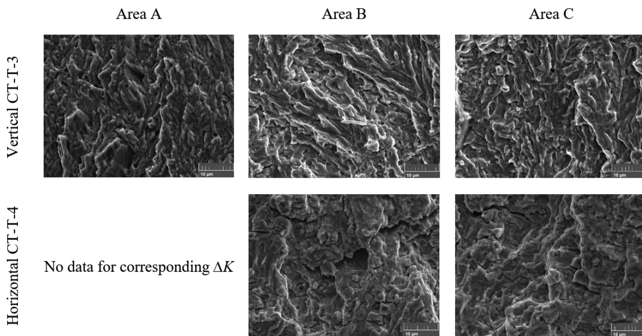
FIGURE 8 SEM fractographs of three areas on vertical (CT-T-3) and horizontal (CT-T-4) specimens with 5,000 magnification (the scale bar is 10 \mu\text{m} , and the right-hand side arrow shows the direction of the crack propagation)
