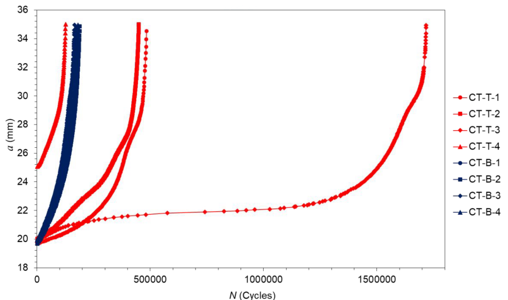
FIGURE 3 Fatigue crack growth trends in ER100S-1 WAAM built specimens extracted from different locations [Colour figure can be viewed at wileyonlinelibrary.com ]
