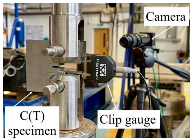
FIGURE 2 Fatigue crack growth test set-up [Colour figure can be viewed at wileyonlinelibrary.com ]
