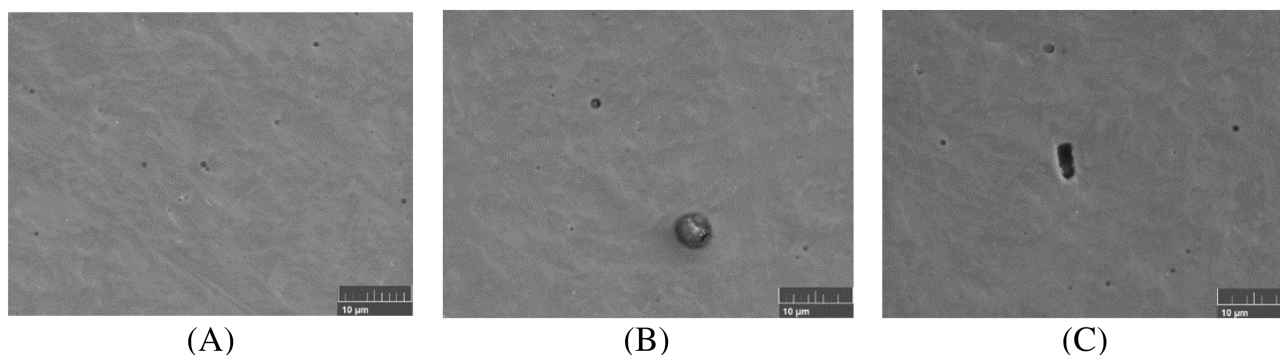
FIGURE 11 SEM fractographs of polished ER100S-1 specimens with defects (A) and (B) gas-entrapped pores and (C) pores and a keyhole porosity defect (the scale bar is 10 µm)
