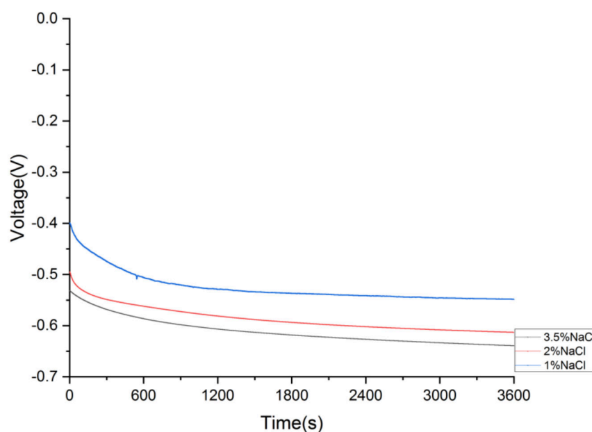
Figure 7. Potential is plotted against time for 1%, 2%, and 3.5% NaCl concentrations at 25 °C when the flow velocity is kept at zero.
