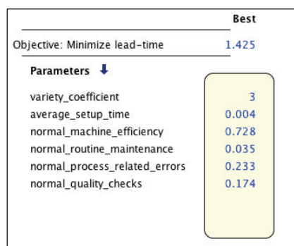
Fig. 7. Snapshot of results of optimization experiment for lead-time minimization
