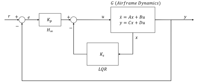
Fig. 2. Control Topology
