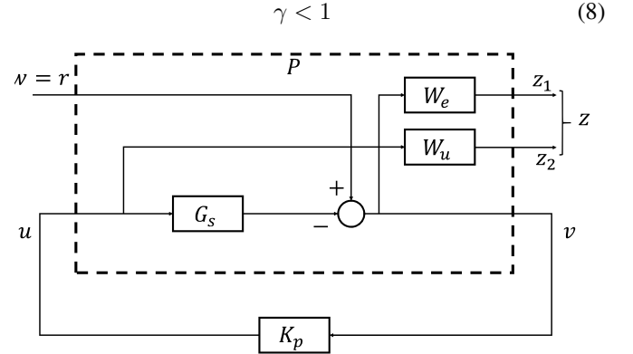
Fig. 5. Mixed-Sensitivity Optimisation Problem
