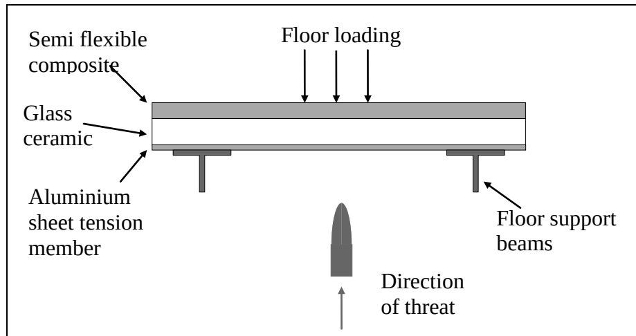
Figure 2. The structure of a proposed structural armour.
