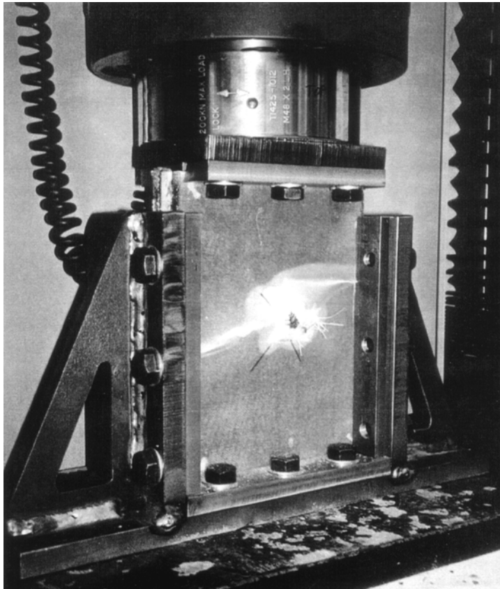
Figure 6. CFRP structural armour panel failing in compression after ballistic impact.
