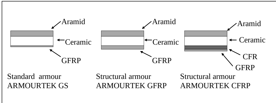
Figure 3. A comparison of the standard and structural armour layouts.
