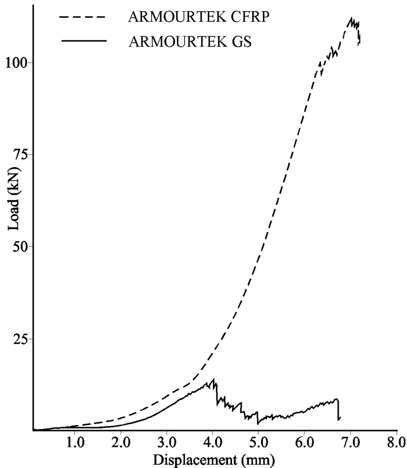
Figure 5. Compression after impact response of standard and structural armour systems.
