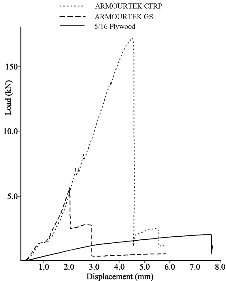
Figure 4. Load displacement plots for test coupons of plywood, standard armour and CFRP structural armour.
