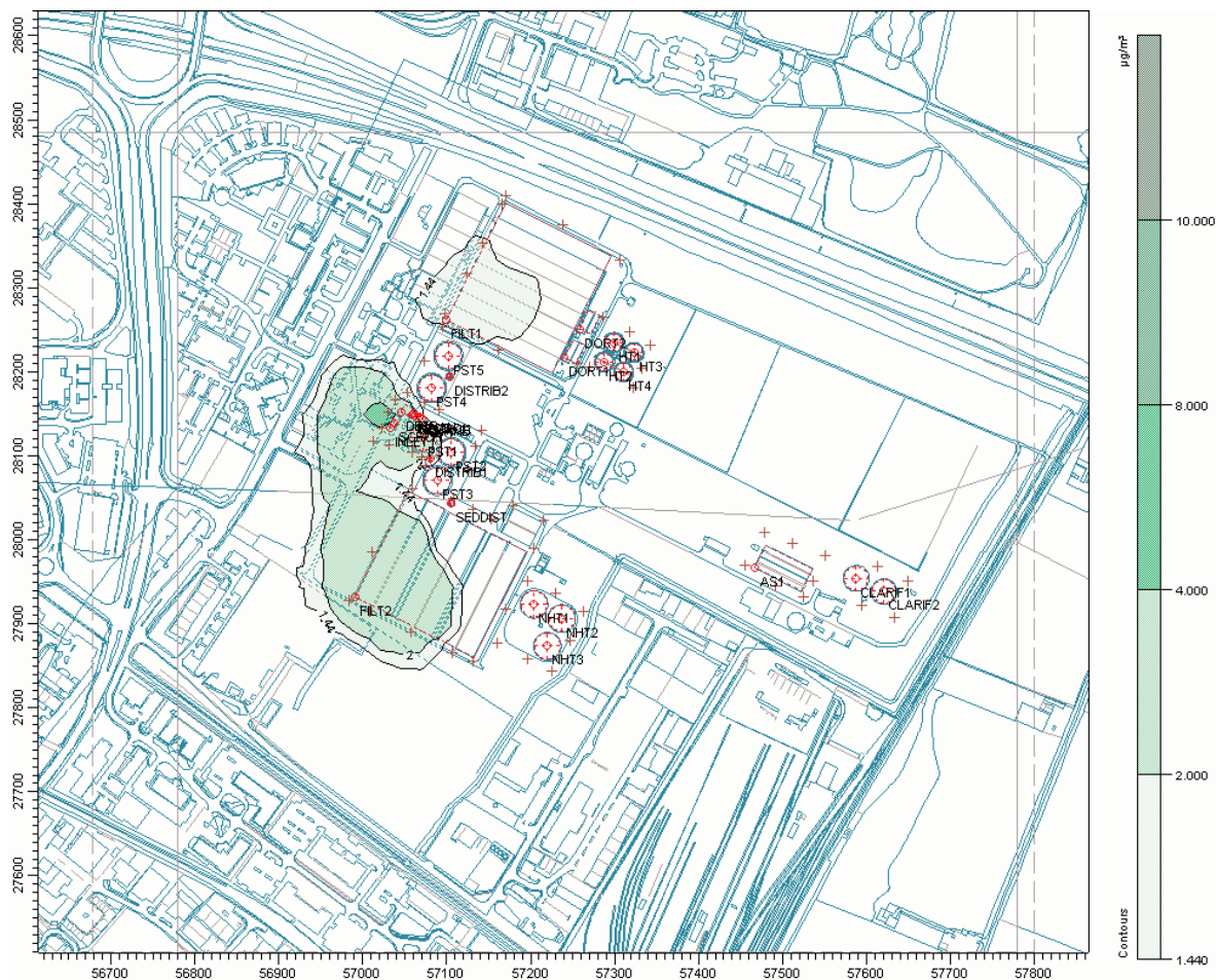
Figure 1: Contour Plot Fitted Micrometeorological Survey Day 1
