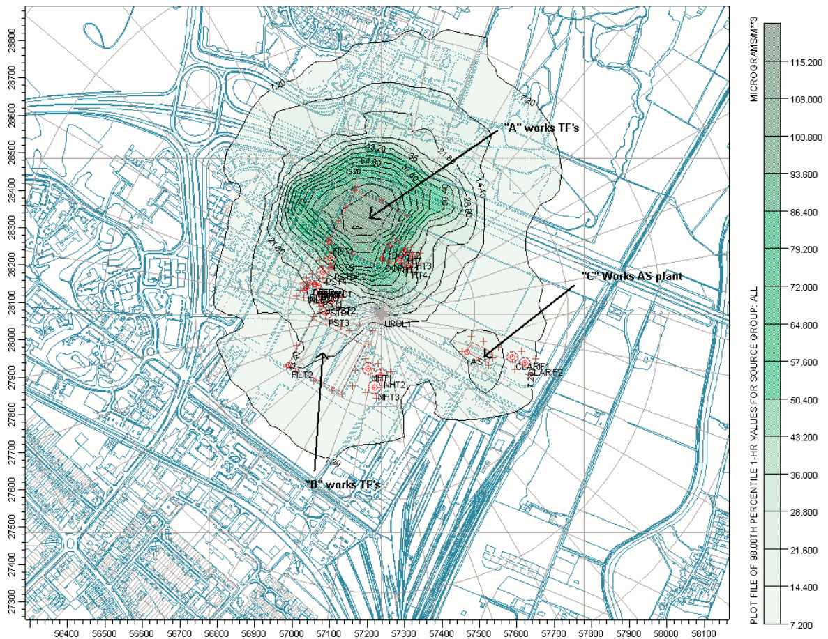
Figure 10: 98%ile Contour plot 2004 Constant emission rate
