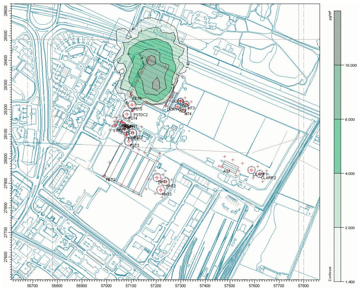
Figure 6: Contour Plot LUT “typical” emissions Day 2
