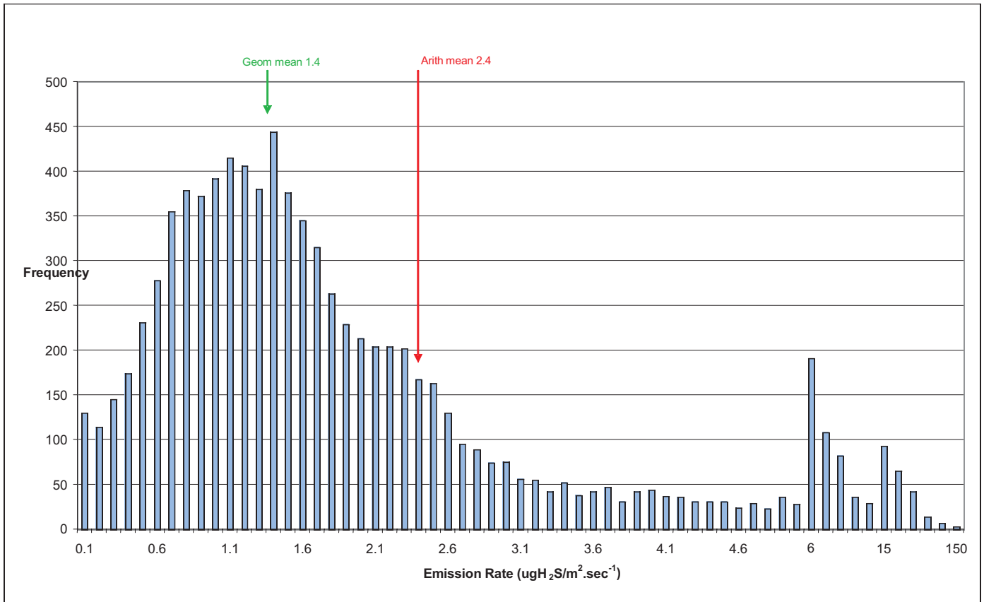
Figure 8: Statistical analysis of “B” Works Trickling filters hourly emission rates
