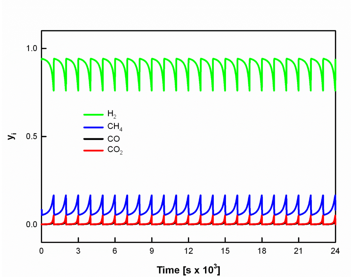
Figure 9 - Gas molar fractions at the outlet of reactor network as a function of the time.
