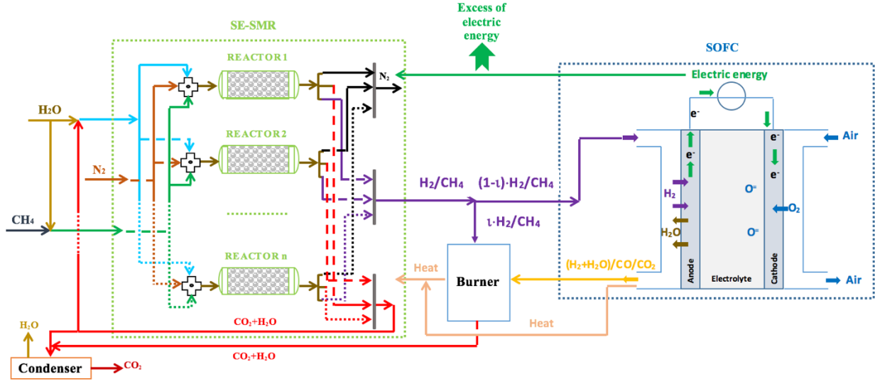
Figure 2 - Schematic layout of the SE-SMR process integrated with a SOFC.
