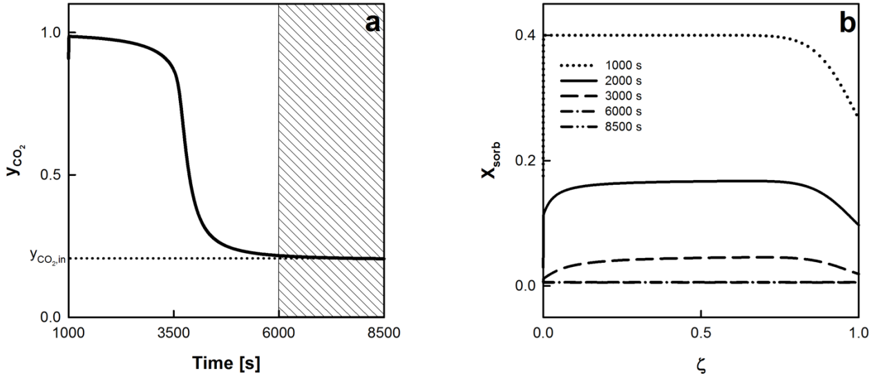
Figure 5 - Outlet CO 2 molar fractions (a) as function of the time and (b) sorbent conversion degree at different times during the first calcination stage. The time horizon starts at the end of the previous CS (1000 s).
