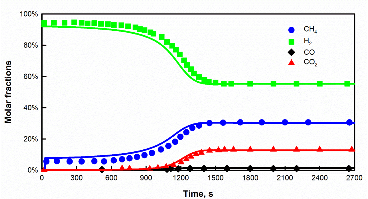
Figure 3 - Literature (dots, [24]) and simulated (lines) outlet gas molar fractions as function of time.
