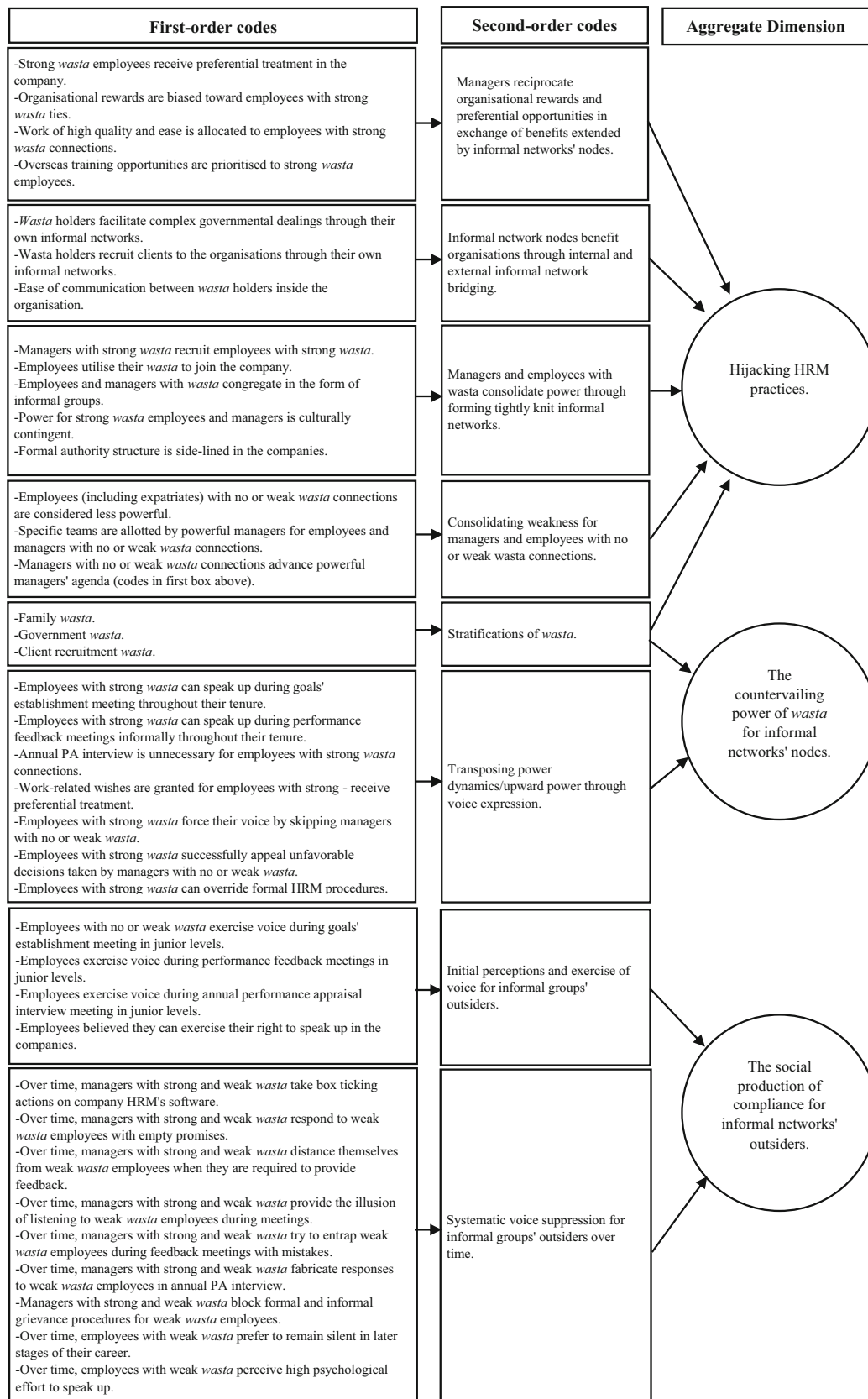
FIGURE 1 Data structure.
