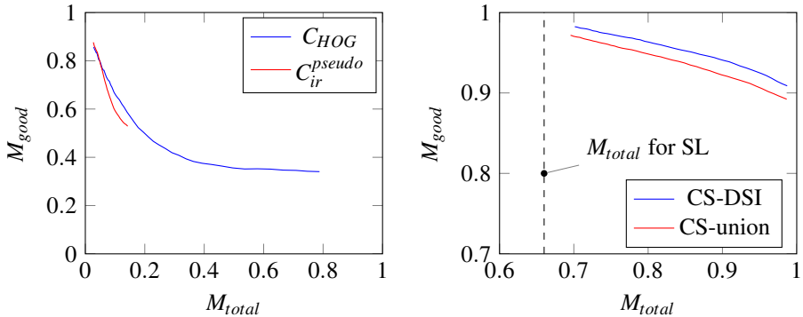
(a) Good match ratio vs. total matches ratio for different matching costs, u = \{0 \rightarrow 0.4\}
