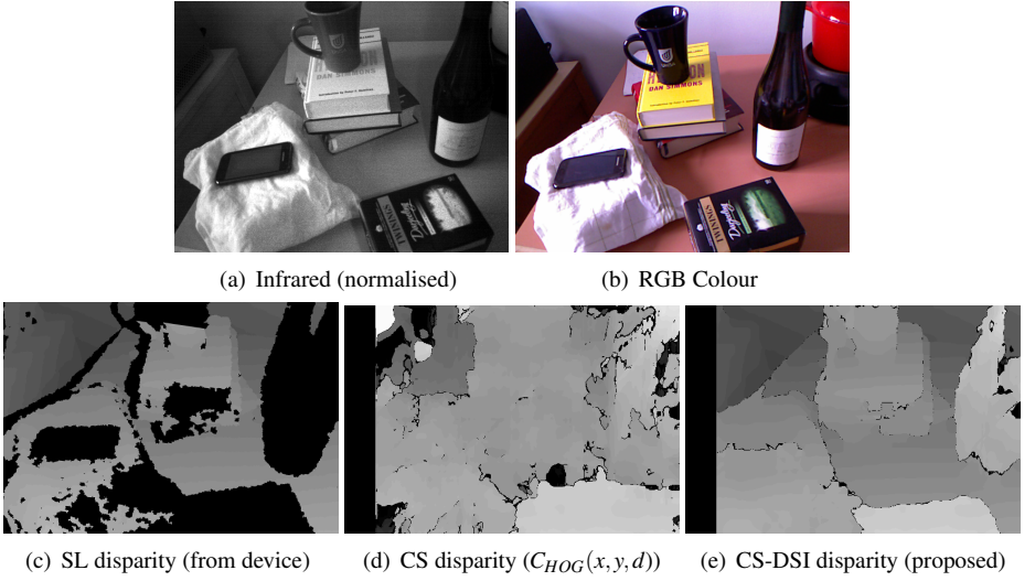
Figure 1: Fused disparity estimation:- ( SL, CS ) \rightarrow CS - DSI
