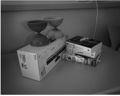
(a) Infrared (normalised)
