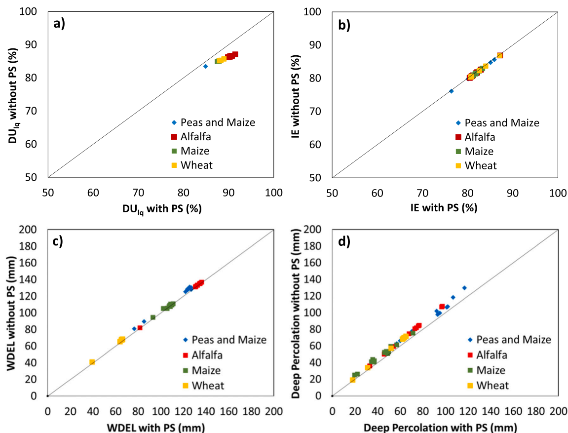
Fig. 10. Comparison of average seasonal irrigation performance indicators (DU iq , IE, WDEL and deep percolation in subfigures a, b, c and d, respectively) between network designs with and without pumping station (PS) at the Bardenas XI WUA. Crops are represented in different colors.
