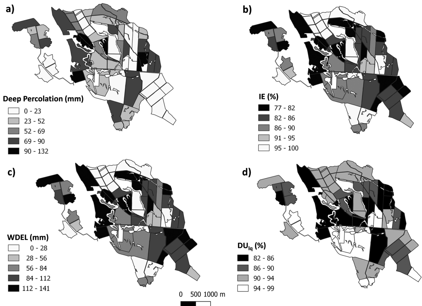
Fig. 9. Average annual irrigation performance indicators for the time data series (2004–2018) of the irrigated area: a) Deep percolation, b) Irrigation Efficiency (IE), c) Wind Drift and Evaporation Losses (WDEL) and d) Distribution Uniformity of the low quarter ( DU_{lq} ) are presented.
