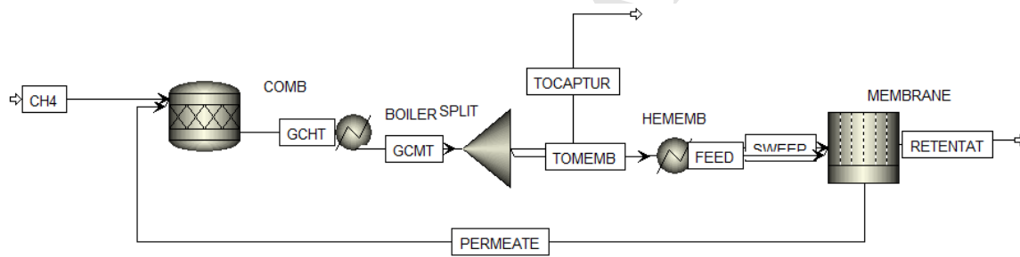
Fig. 5. Aspen Plus interface for membrane model
