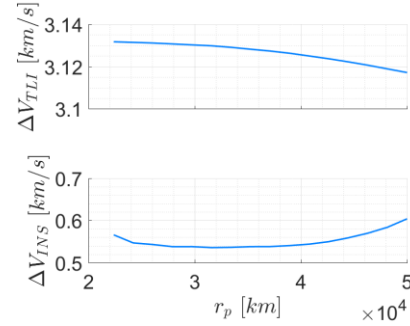
Figure 10. Direct transfers from LEO (200x200 km) to the perilune of L_1 halo orbits. Translunar injection and insertion costs as a function of r_p .
