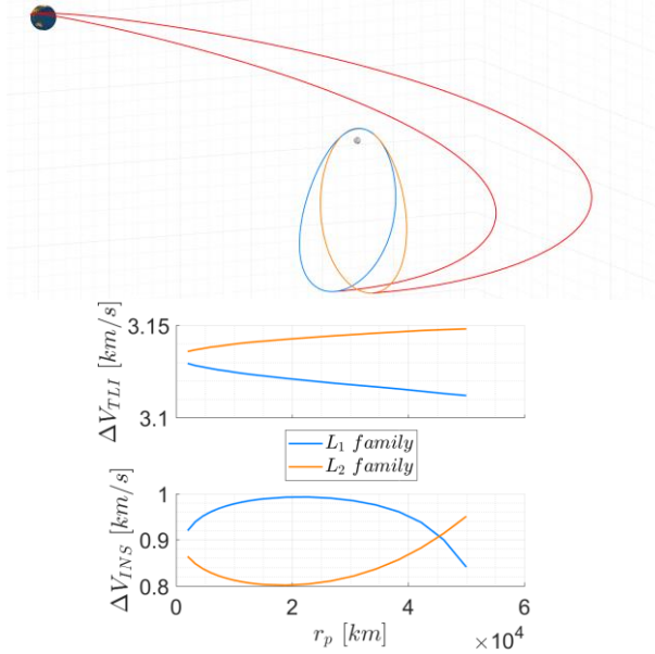
Figure 8. Direct transfers from LEO (200x200 km) to the apolune of halo orbits. Translunar injection and insertion costs for the whole range of L_1 and L_2 halo families as a function of r_p (bottom), and geometry of sample trajectories to NRHOs of r_p = 6,000 km (top) are shown.
