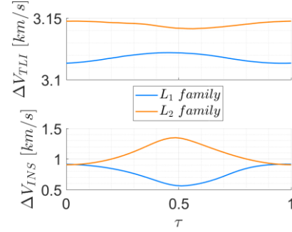
Figure 9. Direct transfers from LEO (200x200 km) to arbitrary points of halo orbits. Translunar injection and insertion costs as a function of \tau for halo orbits of r_p = 45,000 km.
