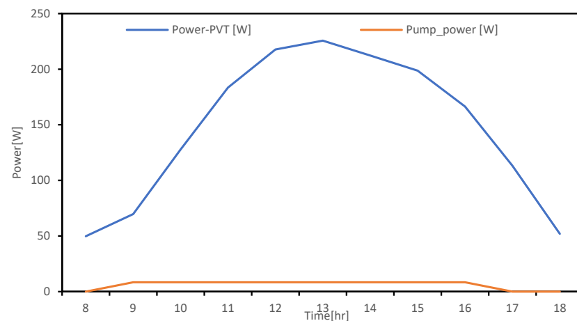
Figure 12. Power output of the PVT system and power consumed by the pump.
