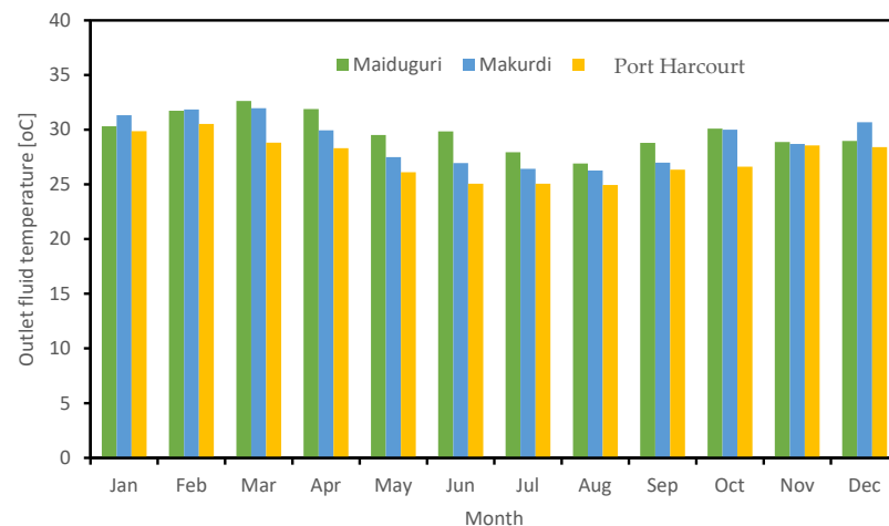
Figure 9. Monthly average outlet fluid temperatures of the three locations in Nigeria.
