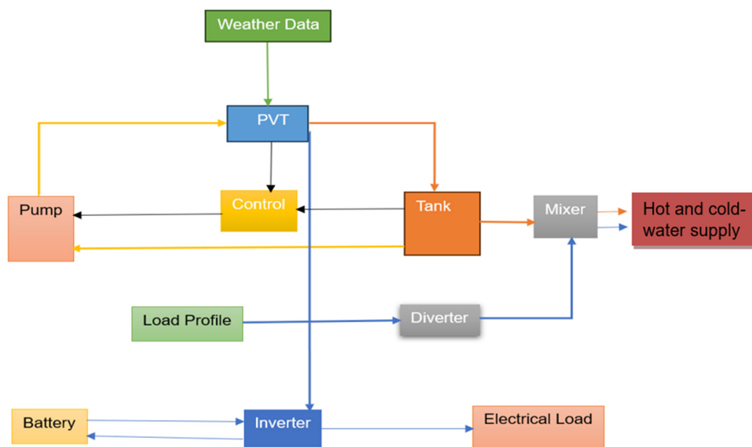
Figure 2. Block diagram of PVT system design.
