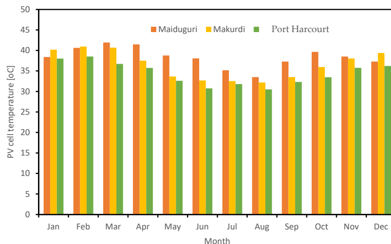
Figure 10. Monthly average PV surface temperature of the three locations in Nigeria.
