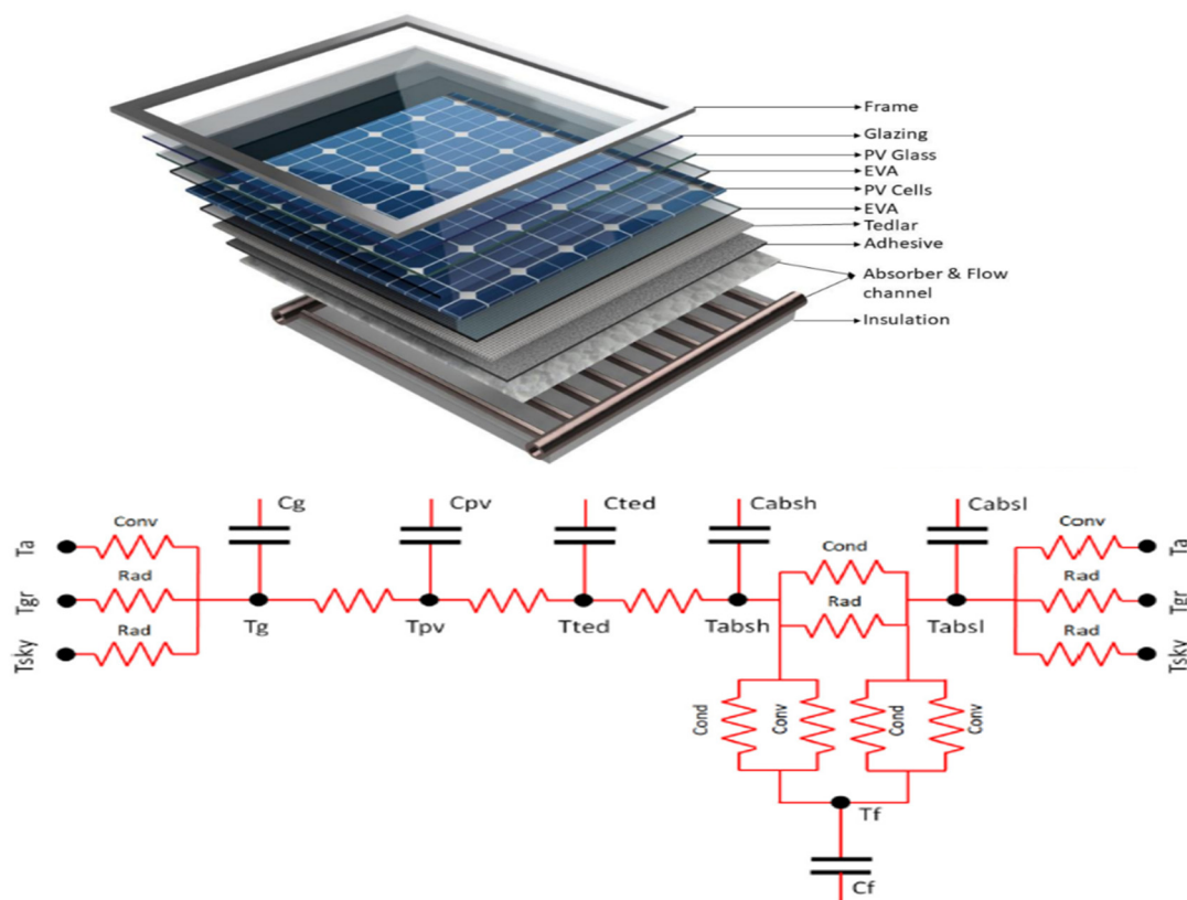
Figure 1. Detailed parts of water-based and equivalent electrical circuit of PVT system [20].
