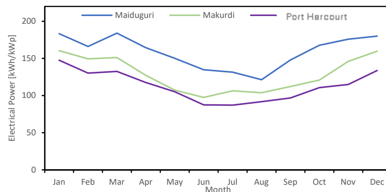
Figure 5. Monthly average peak electrical power outputs in the three locations in Nigeria.
