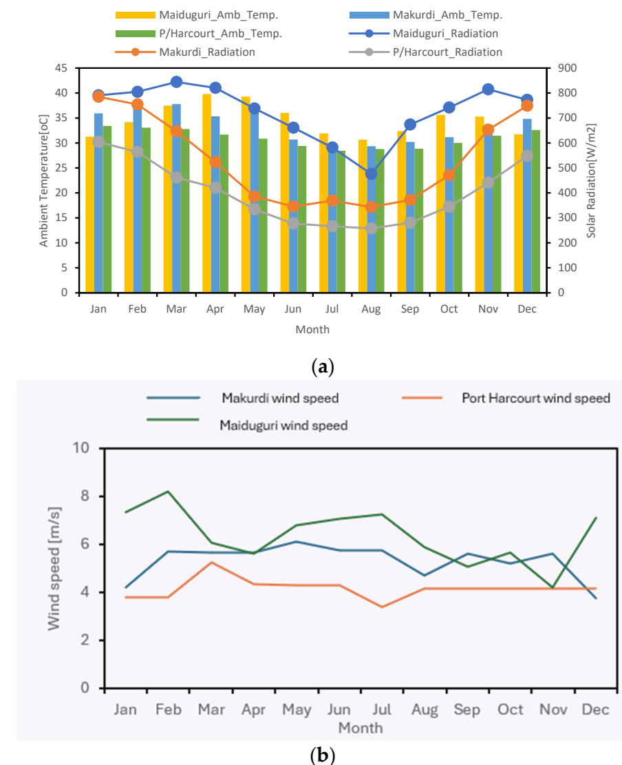
Figure 4. (a) Solar radiation and ambient temperature monthly average of the three locations in Nigeria. (b) Wind speed monthly average of the three locations in Nigeria.
