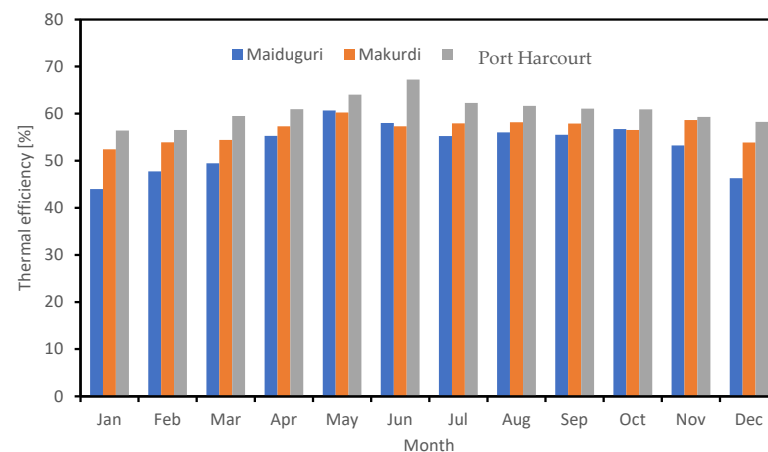
Figure 8. Monthly average thermal efficiencies of the three locations in Nigeria.
