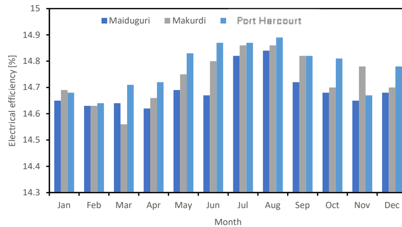
Figure 7. Monthly average electrical efficiencies of the three locations in Nigeria.
