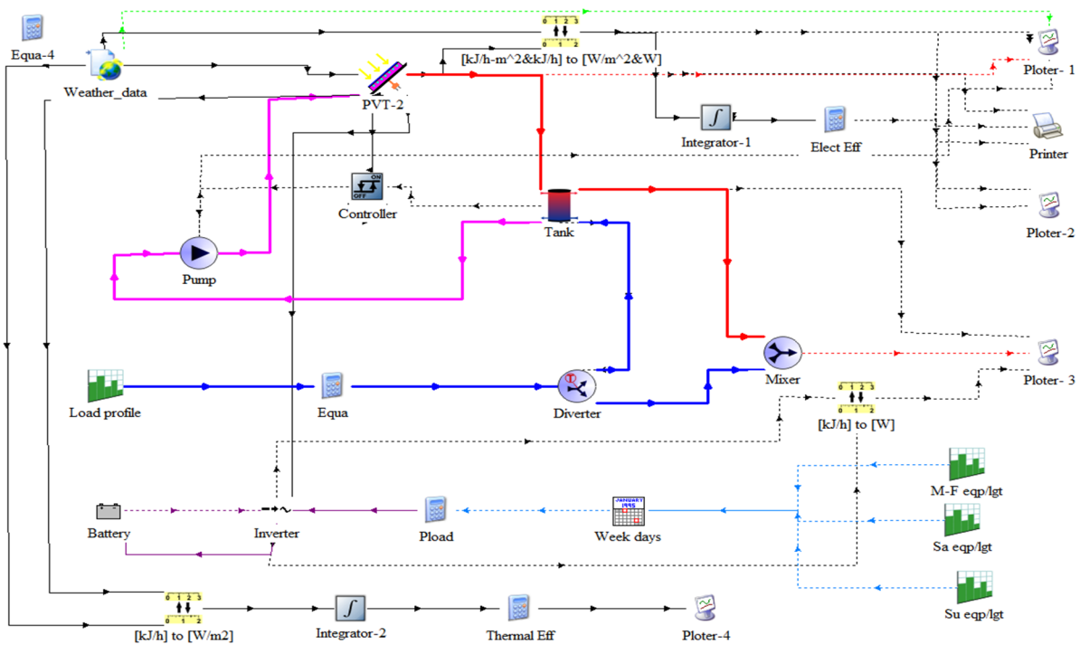
Figure 3. The TRNSYS simulation model of the PVT system design.
