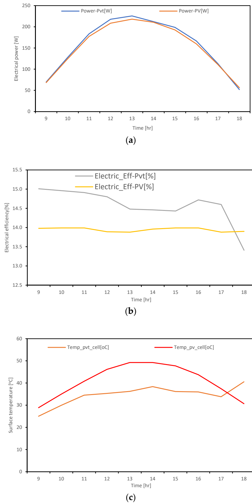
Figure 11. (a) Hourly power outputs of PV panel and PVT system in a day. (b) Hourly electrical efficiency of PV panel and PVT system in a day. (c) Hourly surface temperature of PV panel and PVT system in a day.
