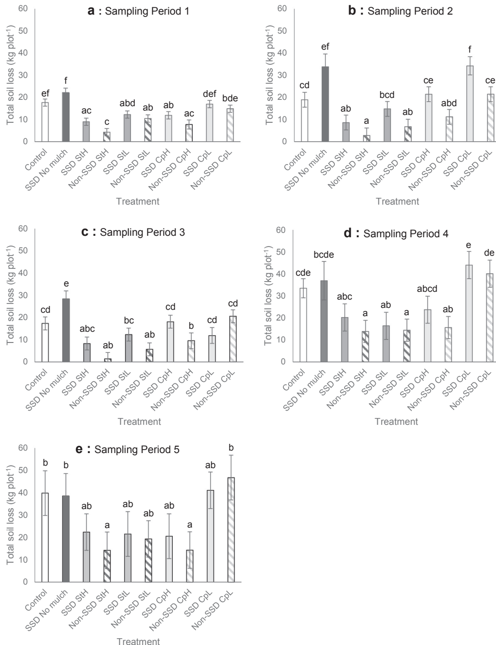
Fig. 2. Mean soil loss (kg plot -1 ) for sampling period 1 (a), period 2 (b) period 3 (c), period 4 (d) and period 5 (e). Error bars show \pm 1 Standard Error. SSD: Treatments with shallow soil disturbance, Non-SSD: Treatments without shallow soil disturbance, Cpl: Compost applied at 8 t ha -1 , CpH: Compost applied at 18 t ha -1 , StL: Straw applied at 3 t ha -1 , StH: Straw applied at 5 t ha -1 . For each sampling period, bars with the same letter are not significantly different ( p \leq 0.05 ) following one-way factorial ANOVA and post-hoc Fisher LSD analysis.
