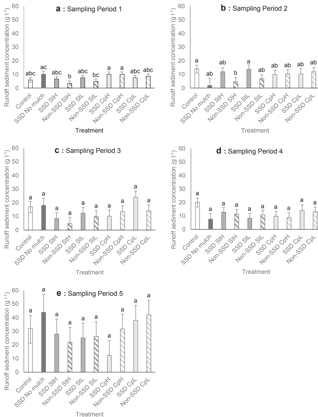
Fig. 3. Mean runoff sediment concentration ( \text{g l}^{-1} ) for sampling period 1 (a), period 2 (b), period 3 (c), period 4 (d) and period 5 (e). Error bars show \pm 1 Standard Error. SSD: Treatments with shallow soil disturbance, Non-SSD: Treatments without shallow soil disturbance, Cpl: Compost applied at 8 \text{ t ha}^{-1} , CpH: Compost applied at 18 \text{ t ha}^{-1} , StL: Straw applied at 3 \text{ t ha}^{-1} , StH: Straw applied at 5 \text{ t ha}^{-1} . For each sampling period, bars with the same letter are not significantly different ( p \leq 0.05 ) following one-way factorial ANOVA and post-hoc Fisher LSD analysis.
