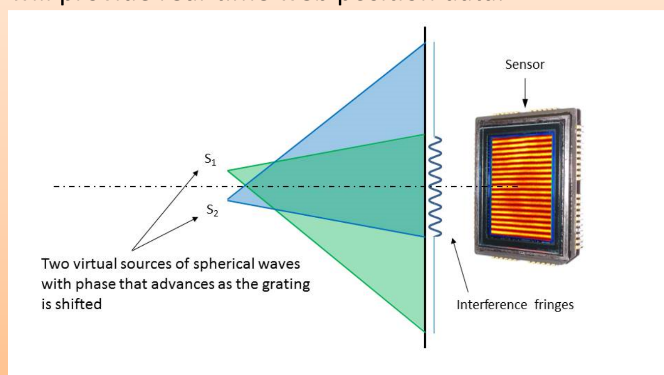
Figure 3: Principle of operation of the NPL linear encoder [2]
