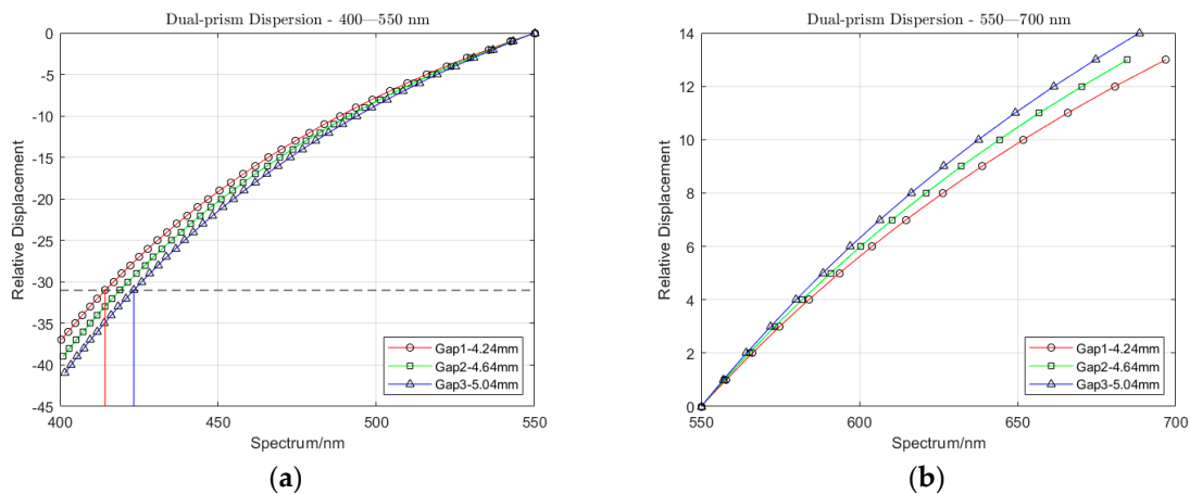
Figure 4. The dispersion of the dual-prism for three air gaps of 4.24 mm, 4.64 mm, and 5.04 mm in the spectral region of: (a) 400–550 nm, (b) 550–700 nm. The y -axis presents the location of pixels along the dispersion plane with respect to the pixel that senses the 550 nm wavelength (the central wavelength position) which is set at 0 mm.
