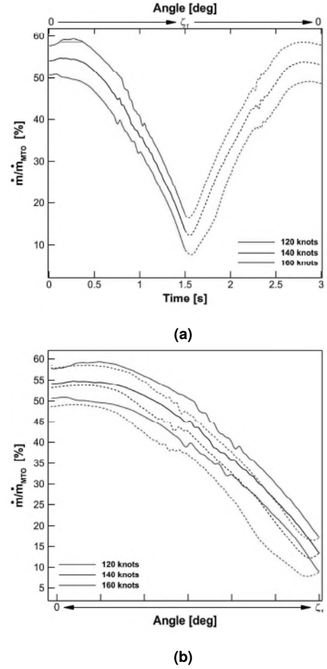
FIGURE 13: Effect of aircraft landing speed on the VPF hysteresis loop: Figure (13a) shows the mass flow rate percentage evolution over time while Figure (13b) shows the VPF hysteresis loops. The forward-to-reverse thrust operations are depicted by solid lines while dashed lines represent the reverse-to-forward thrust operations.
