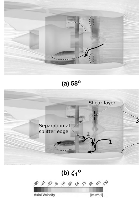
FIGURE 4: Flow field evolution internal and external to the engine when the VPF transitions to reverse thrust mode [16].
