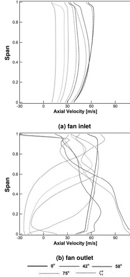
FIGURE 8: Spanwise variation of circumferentially averaged axial velocity at fan inlet (8a) and outlet (8b) for the complete VPF hysteresis loop. The forward-to-reverse thrust operation is depicted by solid lines while dashed lines represent the reverse-to-forward thrust operation.
