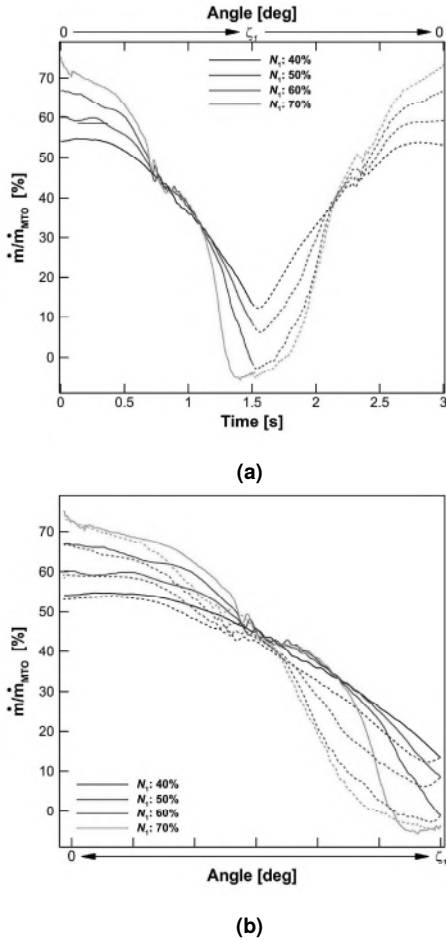
FIGURE 12: Effect of fan rotational speed on the VPF hysteresis loop: Figure (12a) shows the mass flow rate percentage evolution over time while Figure (12b) shows the VPF hysteresis loops. The forward-to-reverse thrust operations are depicted by solid lines while dashed lines represent the reverse-to-forward thrust operations.
