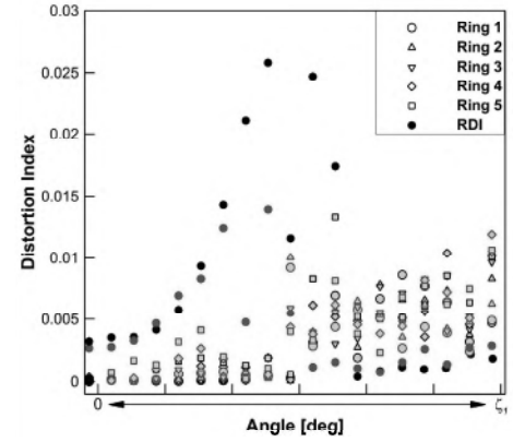
FIGURE 11: CDI and RDI core distortion levels for the complete VPF hysteresis loop. The forward-to-reverse thrust operation is shown in black colour while red colour represents the reverse-to-forward thrust operation.
