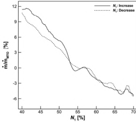
FIGURE 14: Fan rotational speed hysteresis loop: Percentage of mass flow rate evolution ingested by the engine and normalized by the corresponding maximum take-off value.
