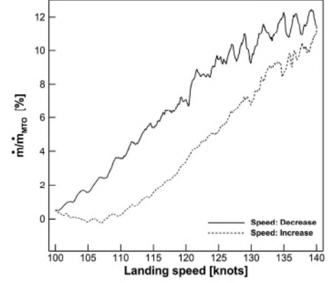
FIGURE 15: Aircraft landing speed hysteresis loop: Percentage of mass flow rate evolution ingested by the engine and normalized by the corresponding maximum take-off value.
