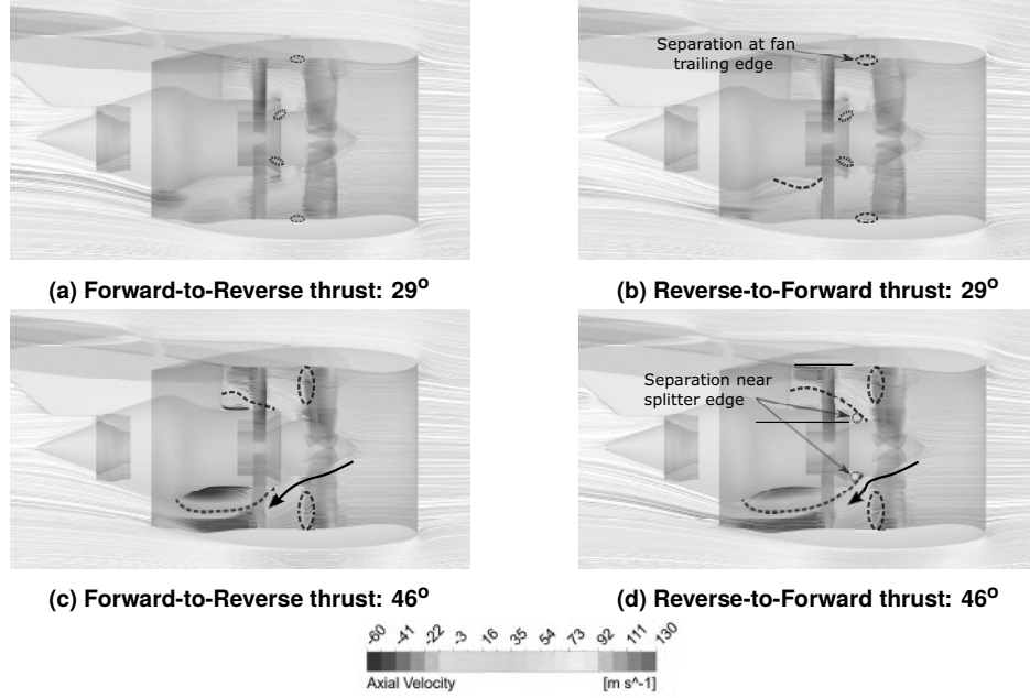
FIGURE 6: Flow field evolution using axial velocity coloured flow streamlines for two timestamp fan stagger angles highlighting the slower dissipation of reverse flow in the reverse-to-forward thrust operation.
