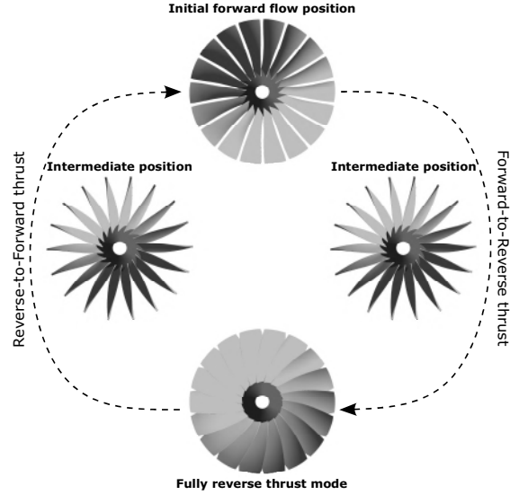
FIGURE 2: VPF blade aerofoils transition from forward flow position to the reverse thrust mode setting and back showing the complete VPF hysteresis loop.
