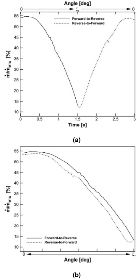
FIGURE 5: Percentage of normalized mass flow rate evolution ingested by the engine. Figure (5a) shows the evolution over time while Figure (5b) shows the VPF hysteresis loop.
