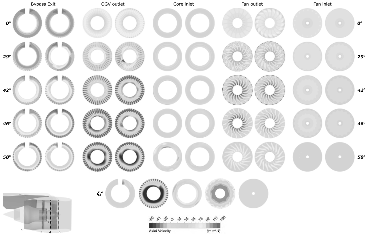
FIGURE 7: Internal flow field development for the complete VPF hysteresis loop using axial velocity contours at five different locations inside the engine for the complete VPF hysteresis loop. The forward-to-reverse thrust operation is represented by the left column at each engine station and the right column shows the reverse-to-forward thrust operation. Core inlet plane is scaled for a more detailed view.
