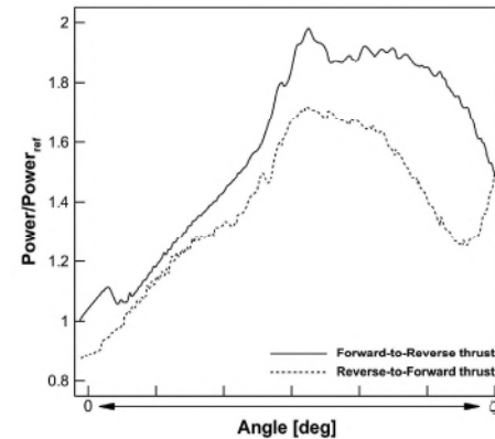
FIGURE 9: Fan power absorption evolution normalised by the nominal forward flow power for the complete VPF hysteresis loop.
