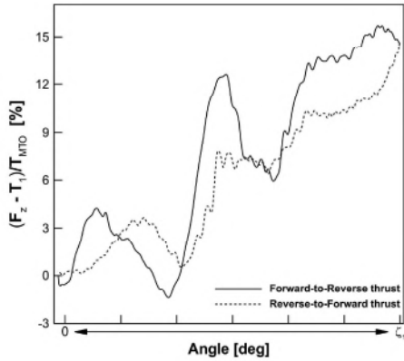
FIGURE 10: Percentage of axial decelerating force evolution normalised by the maximum take-off value for the complete VPF hysteresis loop.
