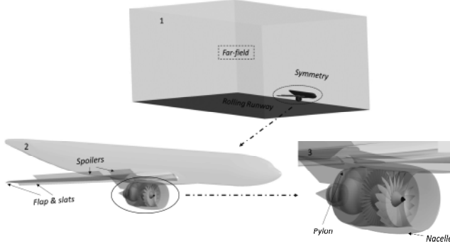
FIGURE 1: Computational domain showing the integrated airframe-engine-VPF model including the engine components [12].
