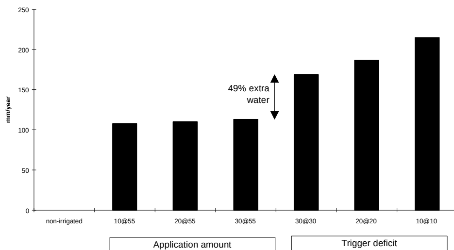
Figure 2 The impact of varying the irrigation plan on average water used for irrigation
