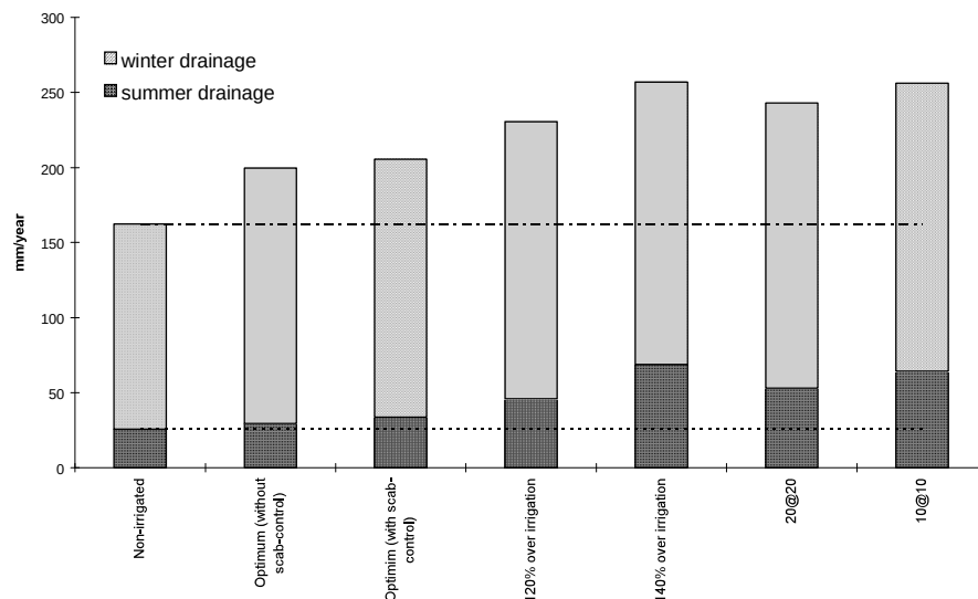
Figure 3 The impact of irrigation schedule of summer and winter drainage
