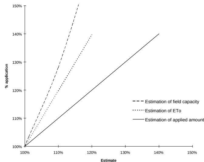
Figure 1 The impact of inaccurate scheduling on water applied
