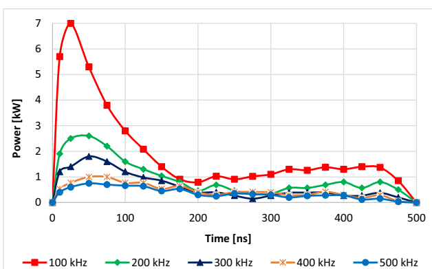
Fig. 5 Pulse shapes of waveform 31 (pulse width of 500 ns) for different pulse repetition frequencies at constant average power of 100W
