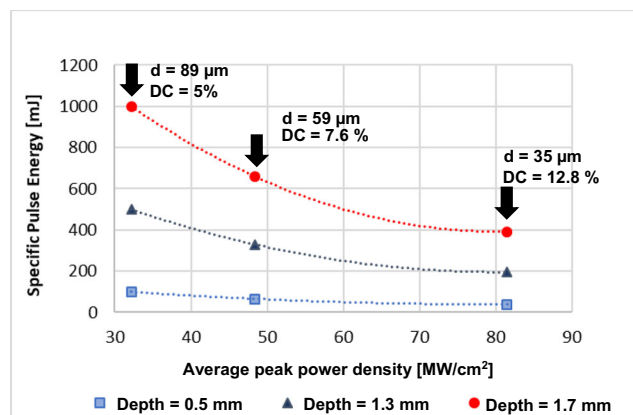
Fig. 7 Specific pulse energy versus average peak power density for depths of penetration of 0.5 , 1.3 and 1.7 \text{ mm} at a constant average power of 100 \text{ W} and pulse width of 500 \text{ ns}
