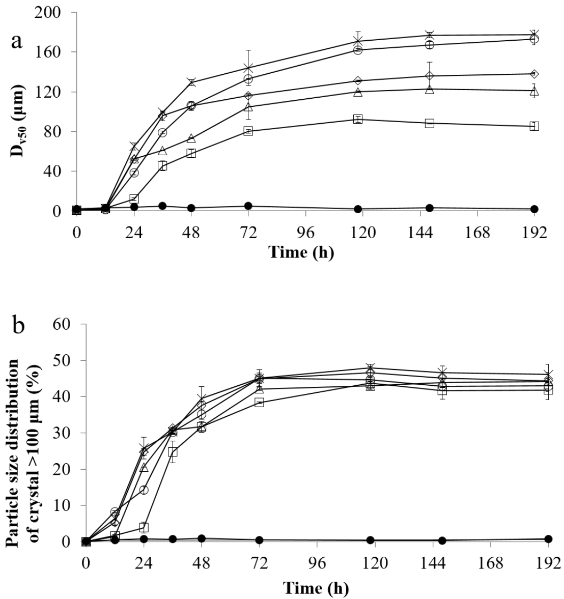
Fig. 4 Variation of D v50 (particle diameter at 50% in cumulative distribution on the basis of volume) (a) and percentage of crystal size >100 μm (b) in the presence of H. salinarum (×), B. antiquum (Δ), B. pumilus (◇), M. xanthus (○) and I. loihiensis (□) in wastewater and non-inoculated controls (●) with time (error bars represent standard deviation obtained from duplicates). D v50 is the value of particle diameter at 50% in the cumulative particle size distribution on a volume basis.
