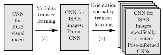
Fig. 5: Training by stage of the Pose-informed CNN. A modality transfer learning followed by an orientation transfer learning.
