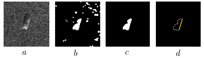
Fig. 2: Contour acquisition and orientation determination of the target. a Original image. b Image after the Gaussian filtering, thresholding, morphological filtering and hole filling. c Small blobs removal. d Orientation of the target contour.
