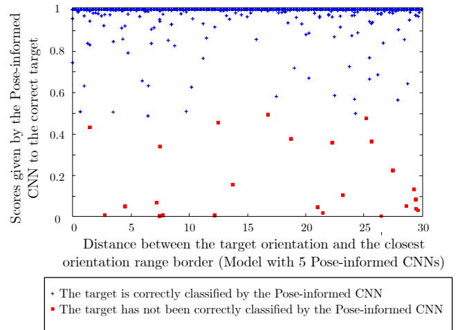
Fig. 8: Analysis of the correct target score and errors according to the distance to the orientation range border on the MSTAR SOC 10 testing set.
