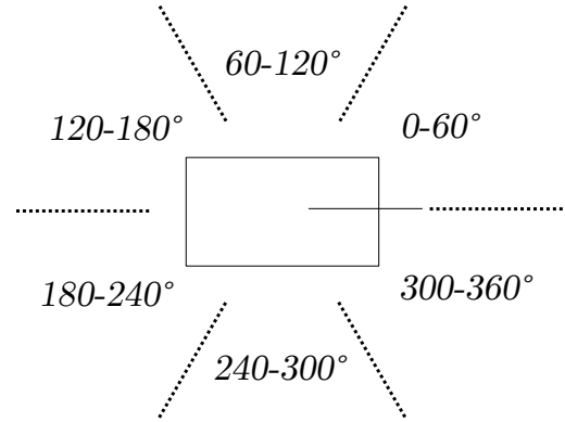
Fig. 4: Orientation ranges for an architecture with 6 Pose-informed CNNs.
