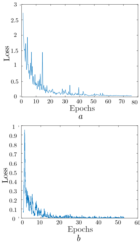
Fig. 6: Evolution of the validation loss during transfer learning. a Evolution of the validation loss during the modality transfer learning of the network. b Evolution of the validation loss during the orientation-speciality transfer learning of the network.
