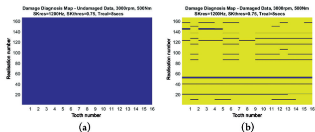
Figure 10. Damage diagnosis maps for 3000 r/min, 500 Nm data when processed with an SK resolution of 1200 Hz and SK threshold of 0.75. The resultant probability of correct diagnosis is 97%: (a) automated diagnosis – undamaged; (b) automated diagnosis – damaged
