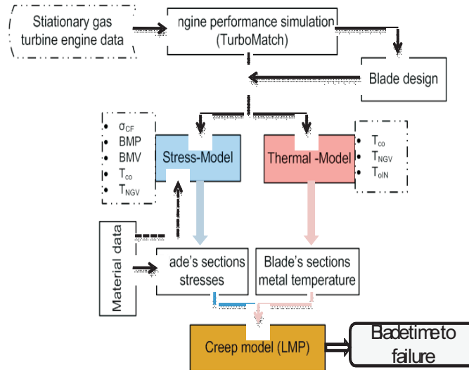
Figure 2 Creep model life assessment
