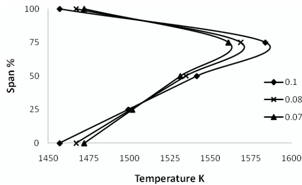
Figure 3 Combustor outlet temperature profile for TET of 1540 K and T_{amb} 318.15 K
