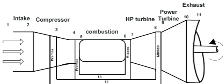
Figure 1 General layout of the engine
