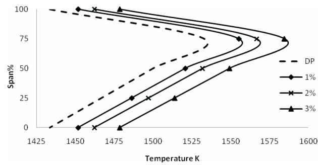
Figure 9 Combustor outlet temperature distribution compressor degradation at T_{amb} 288.15 K
