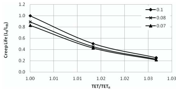
Figure 6 Blade creep life at the root for different RTDF at T_{amb} 288.15 K
