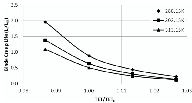
Figure 7 Blade creep life at different T_{amb} for RTDF 0.08
