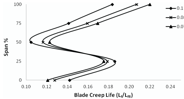
Figure 5 Blade creep life ( L_f/L_{fR} ) along blade span at TET 1540 K and T_{amb} 318.15 K
