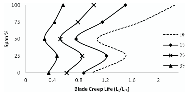
Figure 8 Blade creep life for compressor degradation at T_{amb} 288.15 K
