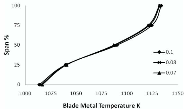
Figure 4 Blade metal temperature distributions along blade span at TET 1540 K and T_{amb} 318.15 K
