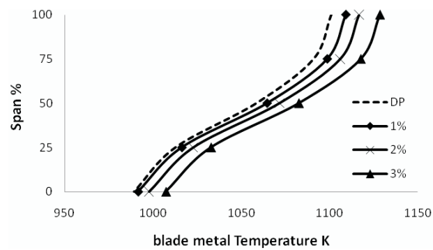
Figure 10 Blade metal temperature compressor degradation at T_{amb} 288.15 K
