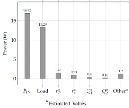
Fig. 10. Power distributions
