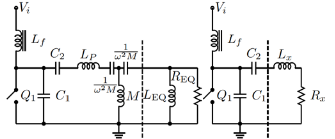
(b) Replacing the Class E rectifier with an equivalent impedance
