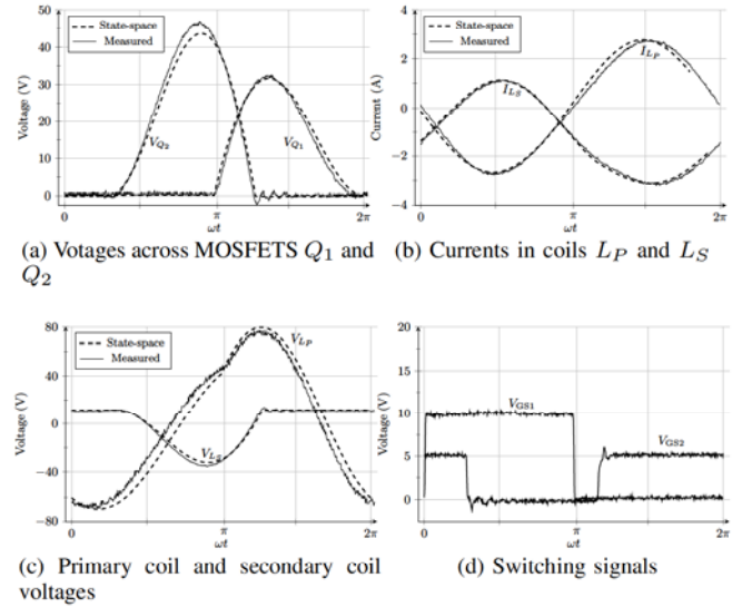
Fig. 9. Measured waveforms
