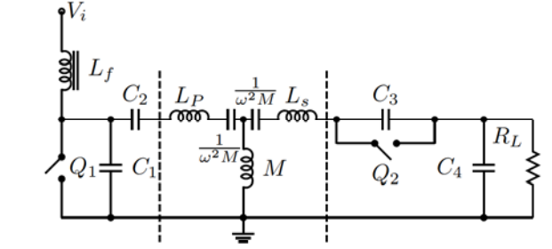
(a) Replacing the inductive link with a T-equivalent circuit
