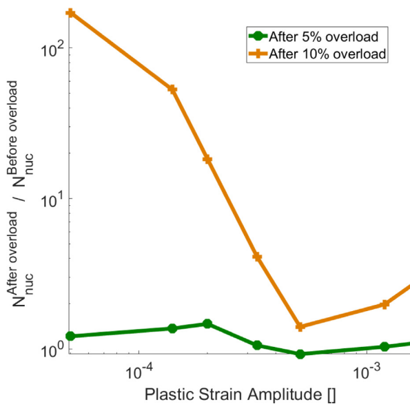
Fig. 12. The effect of the overloads on the fatigue life as a function of the plastic strain amplitude. We used the maximum value of FIP among all elements to consider the most critical fatigue life assessment ( N_{nuc} \propto FIP_{max}^{-2} ). Large enough overloads, modify fatigue life by transforming long structures (Veins, PSBs and Lab.) to cells, which are finer structures.
