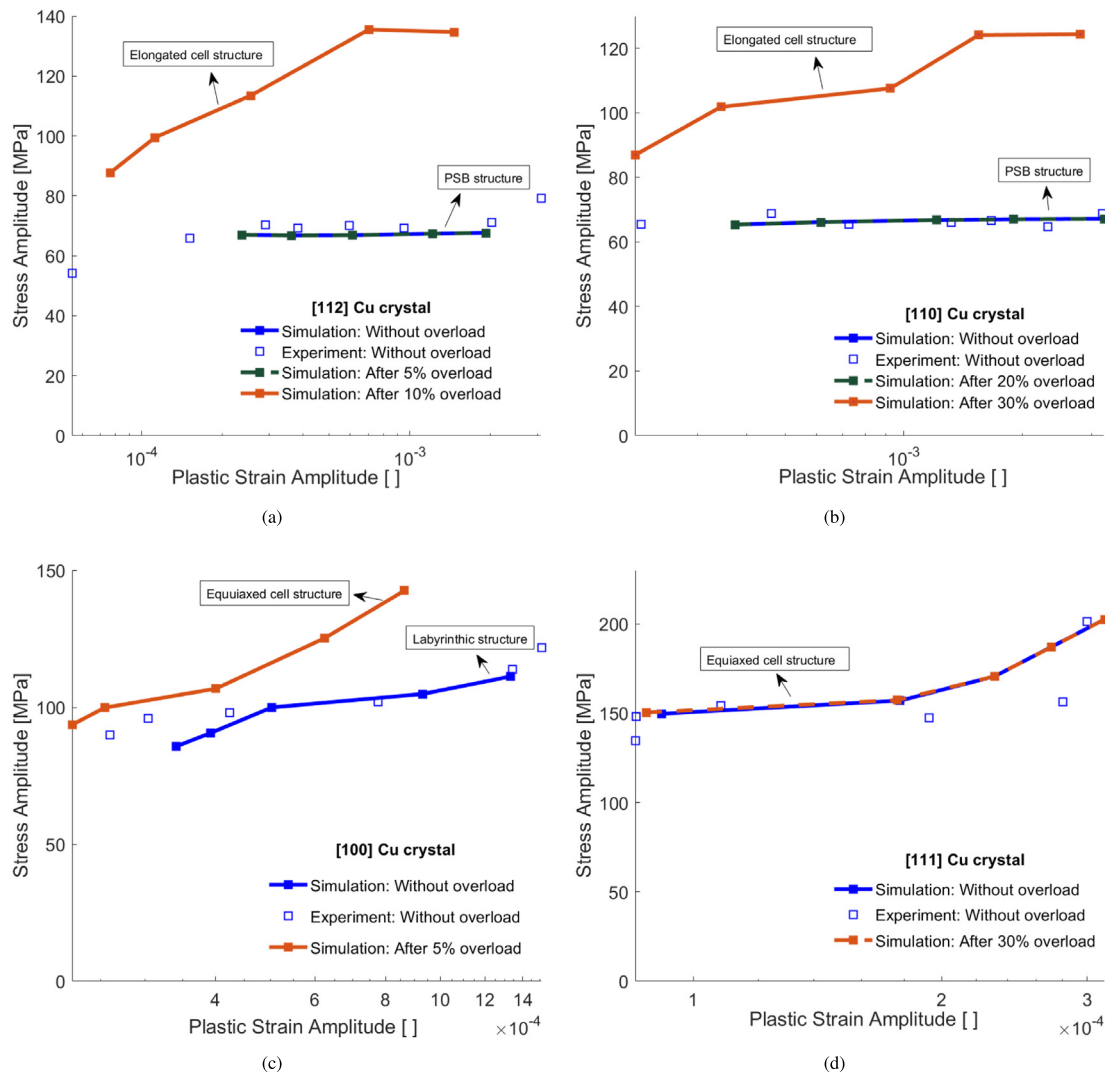
Fig. 9. Predicted effects of overloads on cyclic deformation for (a) [112] (b) [110] (c) [100] and [111] Cu single crystals. While five percent overload is not sufficient to change the structure in [112] crystal, PSBs formed in pre-cycles transformed to elongated cells in ten percent overload. In [110] crystal with longer hardening Stage I, higher overloads are needed to change the structure. Accordingly, PSBs are stable even after 20 percent but altered to elongated cells after 30 percent overload. Labyrinthine structure in [100] crystal is changed to equiaxed cells even in five percent overload. Cell structure in [111] multiple slip crystal is stable even after 30 percent overload and stress remained unchanged. Experiments from Refs. [48–51].
