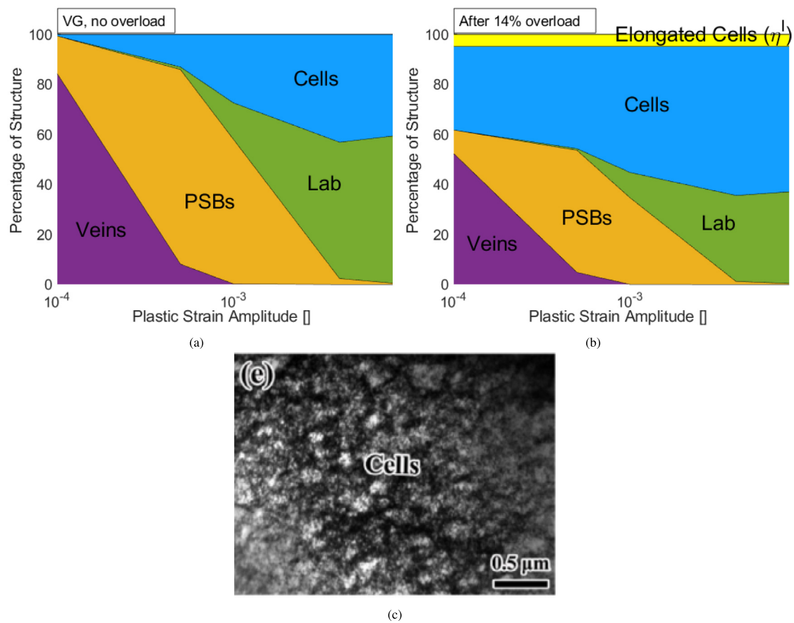
Fig. 8. Predicted mesoscale structures for VG sample (a), and after 14 percent overload (b) and (c) TEM image showing the refined structure after the overload. The transformation of long structures to cells by the overload increases the stress. Experiments from Refs. [2,44].
