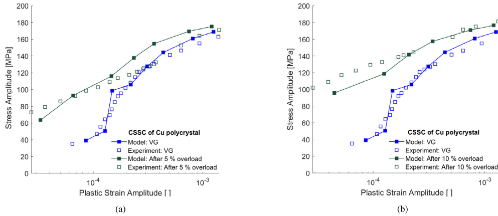
Fig. 5. Increase of saturated cyclic stress of Cu polycrystal and transformation of mesoscale structures by five and ten percent overloads. CSSCs of virgin (VG) Cu polycrystals after (a) Five and (b) Ten percent overload. The macroscopic stress increase by the overloads coincides with mesoscale structure transformations. The experimental data from Ref. [3].
