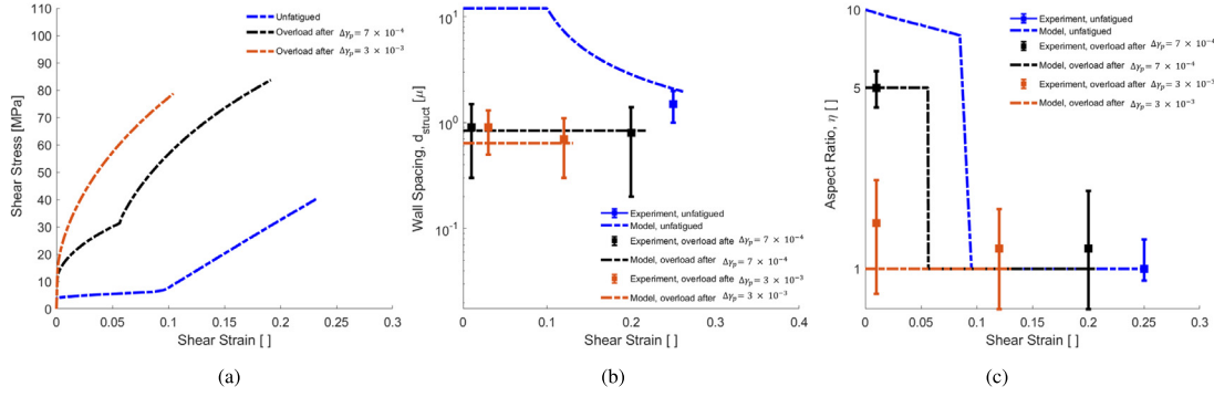
Fig. 4. Meso- and macro-scale overload response of [017] Cu single slip crystal, subjected to different pre-cyclic deformation. Blue, black, and red curves demonstrate the overload response without (unfatigued), after low, and after high cyclic deformation, respectively (low 7 \times 10^{-4} and high 3 \times 10^{-3} cyclic plastic strain, \Delta\gamma_p ). (a) Predicted stress-strain curves, (b) Walls spacing, d_{struct} , (c) Substructure aspect ratio, \eta . Experiments from Ref. [21].
