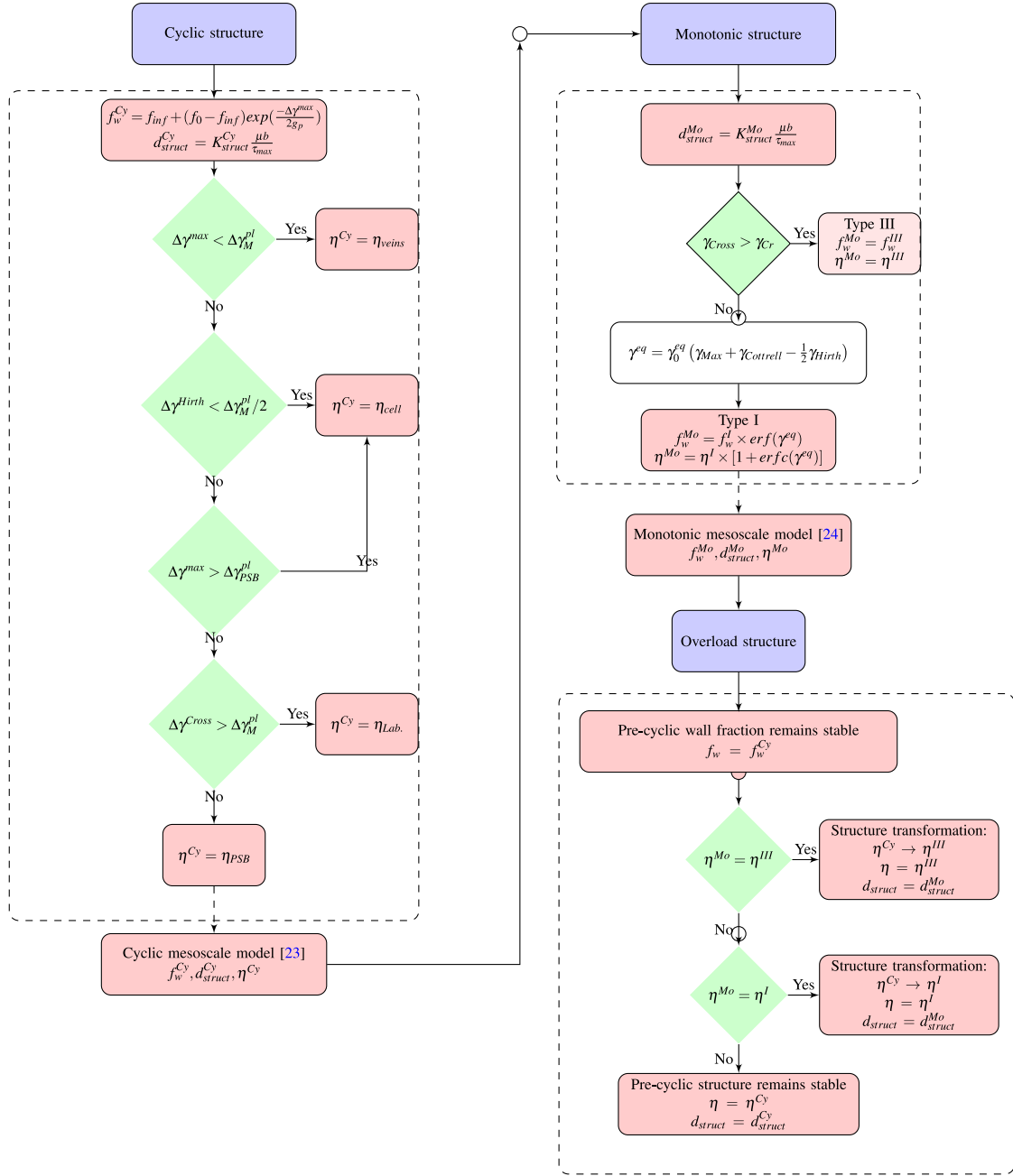
Fig. 1. The cyclic (top left), the monotonic (top right) and the overload (bottom right) models to predict mesoscale structures. The overload model equates that in the post-overload cycles, the pre-cyclic wall fraction remains stable ( f_w = f_w^{Cy} ). If the pre-cyclic structure transforms to Type III or Type I in monotonic model, then it will remain stable in post overload cycles, otherwise, the pre-cyclic structure remain unchanged (no overload effect).
