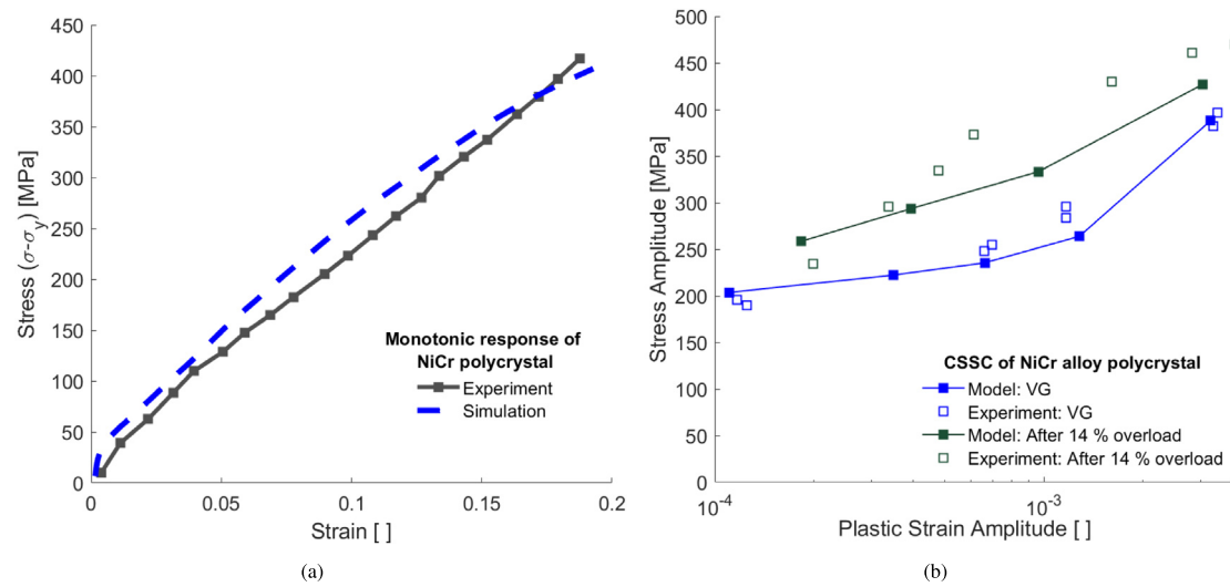
Fig. 7. (a) Prediction of monotonic response of NiCr polycrystal. (b) CSSCs of virgin (VG) material and after 14 percent overload of this alloys. Experiments from Refs. [2,44].
