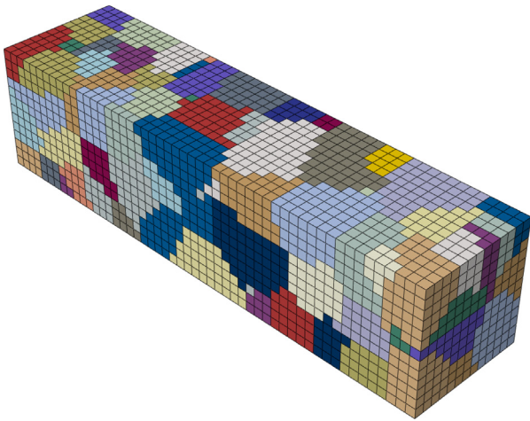
Fig. 3. Realistic microstructure and mesh with 101 equiaxed grains, 8788 elements and uniaxial loading. On one end nodes are restricted to move in the axial direction while on the other end their are displaced under strain control.
