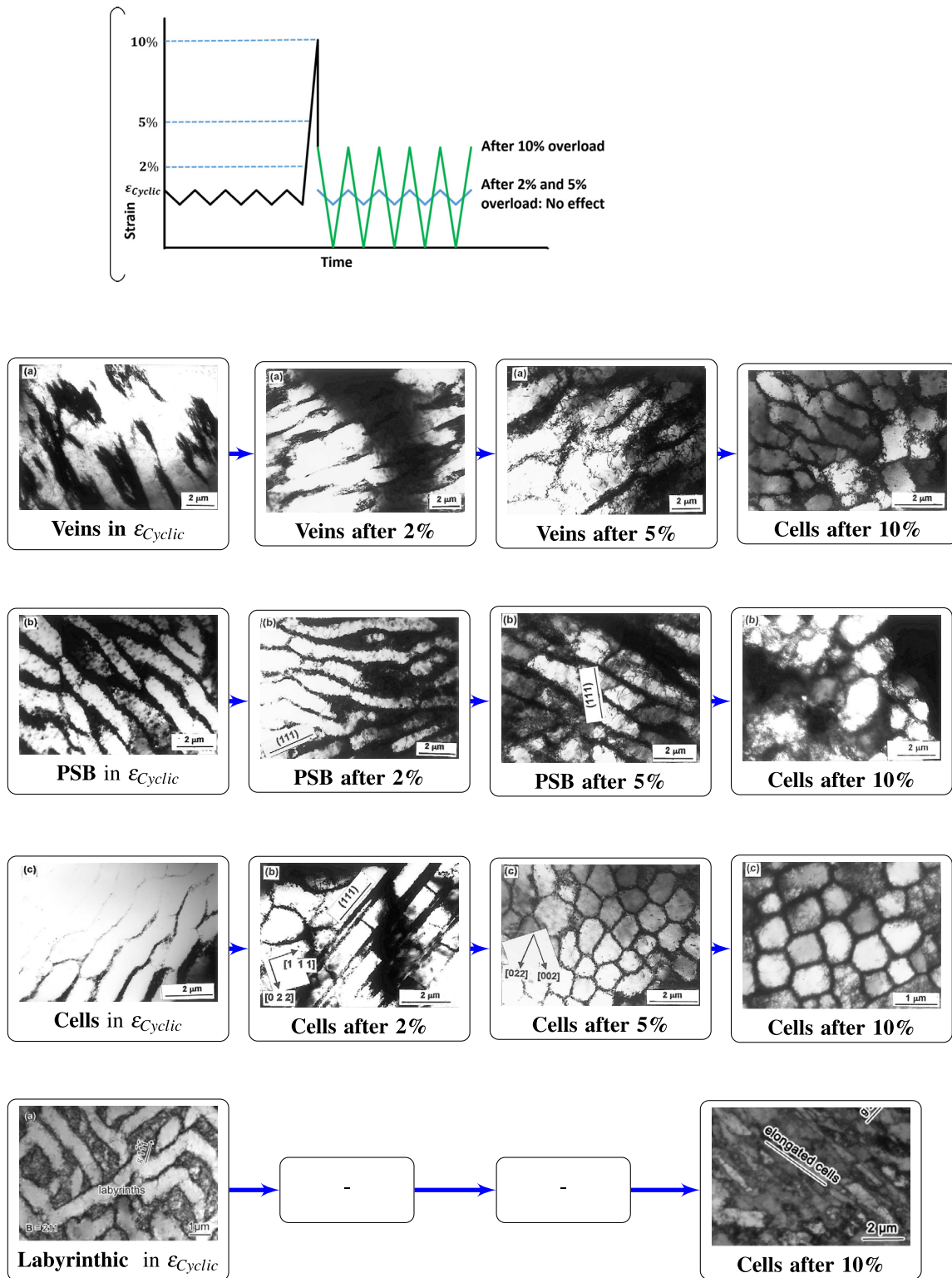
Fig. 2. Stability of various cyclic substructures during overloads. Veins, PSBs and labyrinthine substructures are stable up to five percent and transformed to stable monotonic structures (equiaxed and elongated cells) at ten percent overload. The TEM images from Ref. [4].
