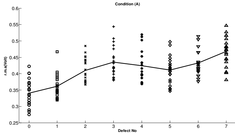
Figure A13 AE r.m.s level associated with defect condition 'A'
