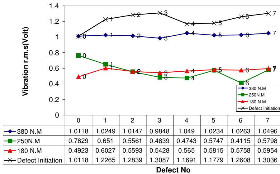
Figure 103 Vibration RMS level for each defect at different loading condition
