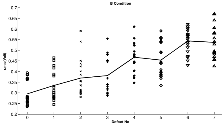
Figure A14 AE r.m.s level associated with defect condition 'B'
