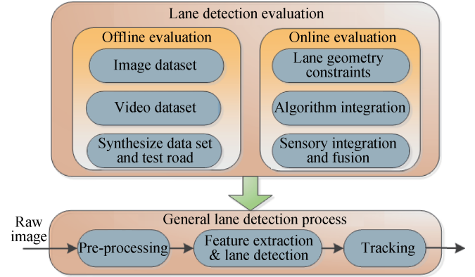
Fig. 3. Lane detection evaluation architecture with two different evaluation methodologies.
