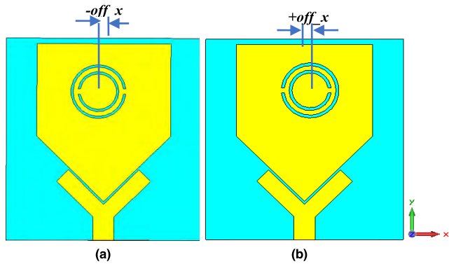
FIGURE 3. Orientation of slits for generation of (a) RHCP, (b) LHCP.
