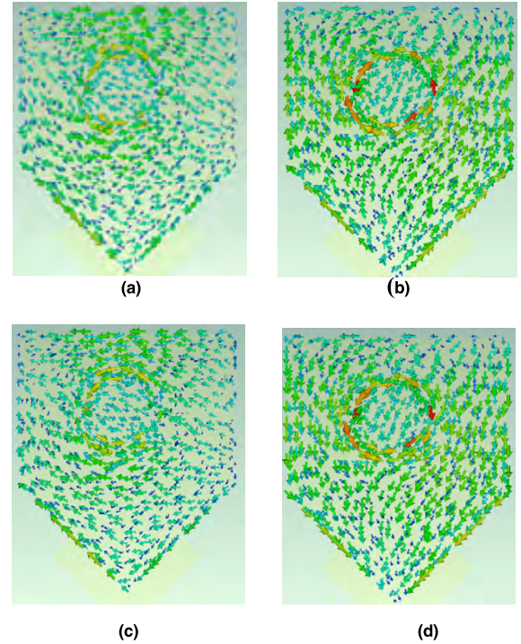
FIGURE 2. Current distribution of the proposed antenna at 1.575 GHz (L1 band) for different time events \omega t (a) 0^\circ , (b) 90^\circ , (c) 180^\circ , and (d) 270^\circ .
