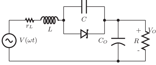
Fig. 1. Circuit diagram of the Class E ZVS low dv_a/dt rectifier with a rectifying diode.
