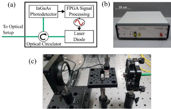
Figure 2. (a) shows a schematic of the hardware used in the paper. (b) shows a photo of the fully enclosed interrogation hardware, while the experimental setup used is pictured in (c).
