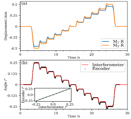
Figure 3. (a) Measured displacements for the two parallel beams incident on the mirror, with the reference interferometer R subtracted, for a series of stepped pitch angle changes. (b) shows the angle change calculated from these displacements measured by the interferometer, compared to data from the pitch motor stage encoder. In the inset in (b), the encoder measurements are plotted directly against the interferometer measurements, with a best linear fit plotted alongside.
