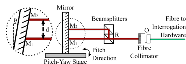
Figure 1. Schematic of the experimental setup used in this paper with reflection points O, R, M_1 and M_2 labelled. A close-up of the mirror incident points is shown on the left showing the pitch angle \theta and the separation of the beams, d .
