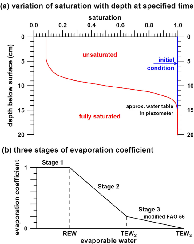
Fig. 1. Features of evaporation (a) experimental saturation curve as evaporation occurs from sand surface (deduced from Smits et al., 2012; Davarzani et al., 2014), (b) FAO approach for reduction in evaporation as water table falls (derived from Mutziger et al., 2005).
