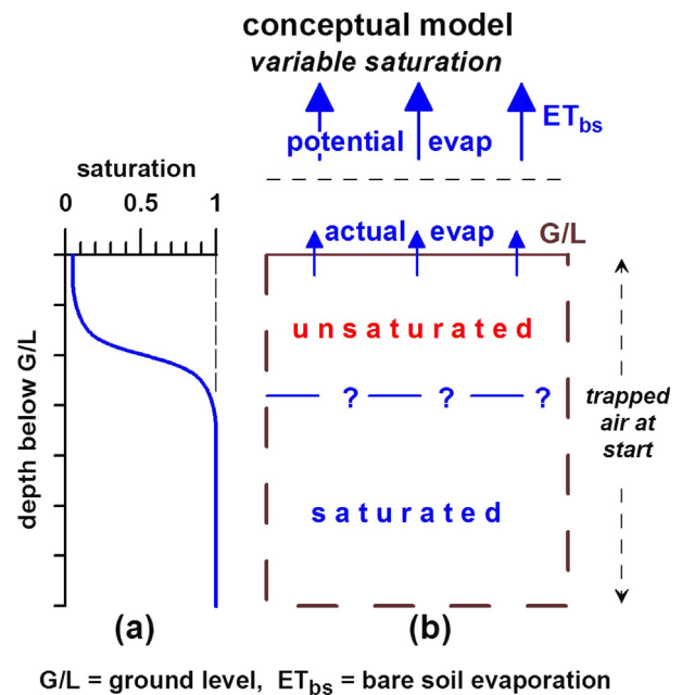
Fig. 3. Conceptual model of conditions in a sand lysimeter as the water table falls due to evaporation.
