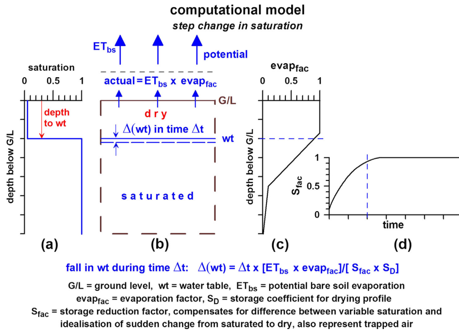
Fig. 4. Computational model for evaporation from a lysimeter containing sand: (a) assumption of sudden change in saturation at water table, (b) actual evaporation and fall in the water table, (c) change of evaporation factor with depth to water table, (d) change of storage reduction factor with time.
