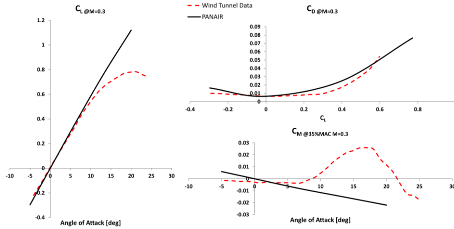
Figure 3 Low speed validation: PANAIR vs wind tunnel data for 1303 UCAV.
