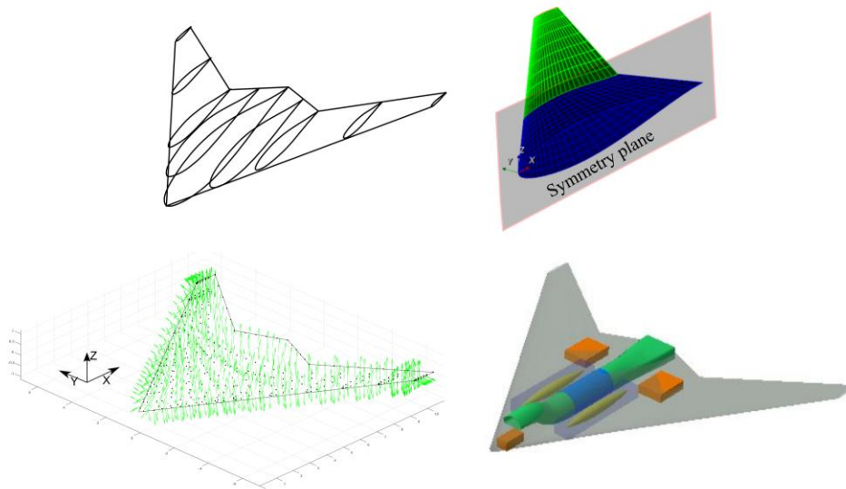
Figure 8 Wireframe, aerodynamic panels, RCS (facet normal vectors), and packaged CATIA geometries
