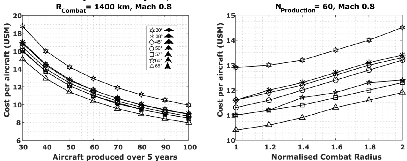
Figure 17 CPA against production number and normalised combat radius
