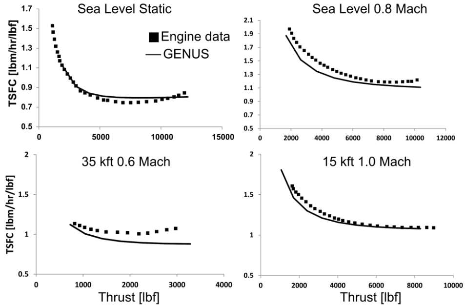
Figure 5 Validation of propulsion models inside GENUS.
