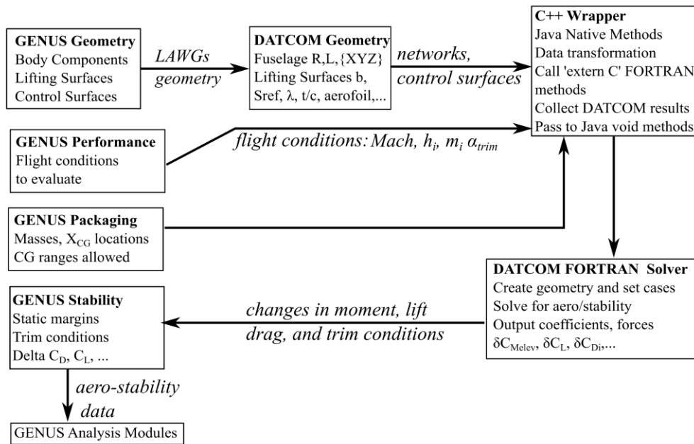
Figure 6 GENUS to DATCOM data sharing and processing.
