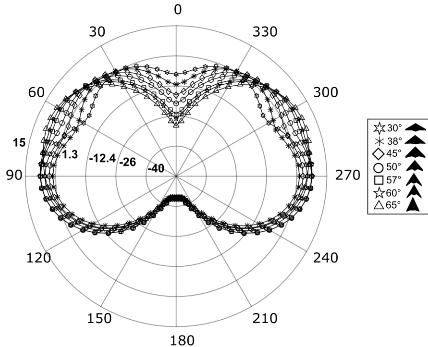
Figure 16 RCS for perfect electric conductor, S band (3 GHz), \theta = 90^\circ \phi = [0^\circ, 360^\circ]
