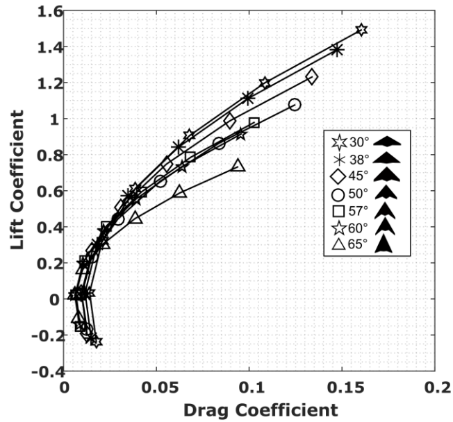
Figure 11 Drag polar for all configurations at Mach 0.8 and cruise altitude.
