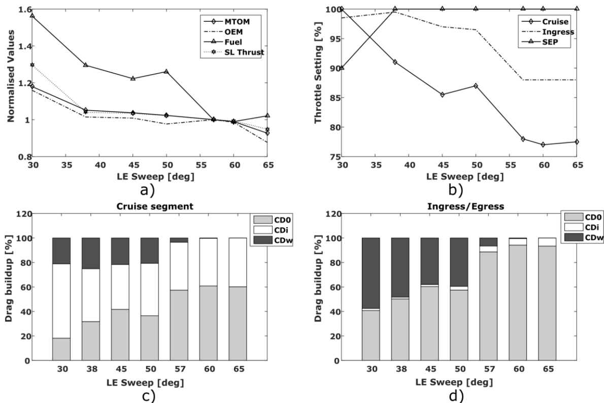
Figure 10 Normalised mass and thrust (a), throttle setting for cruise, ingress/egress, and SEP requirement (b), drag buildup during cruise (c) and ingress/egress segments (d)
