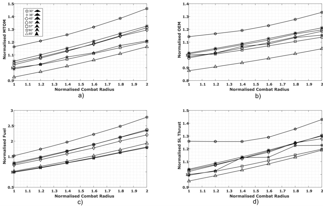
Figure 14 Effect of increasing combat radius ( M_{Cr} = 0.8 ) on MTOM (a), OEM (b), fuel (c), and sea level thrust (d).
