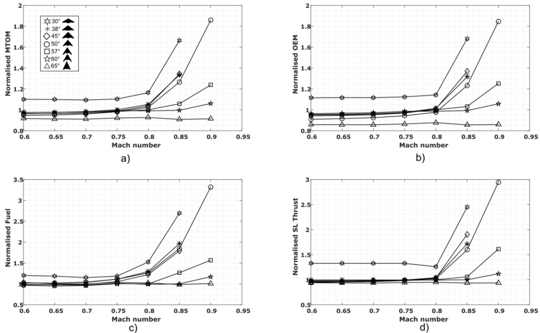
Figure 12 Effects of cruise Mach number on MTOM (a), OEM (b), fuel (c), and sea level thrust (d).
