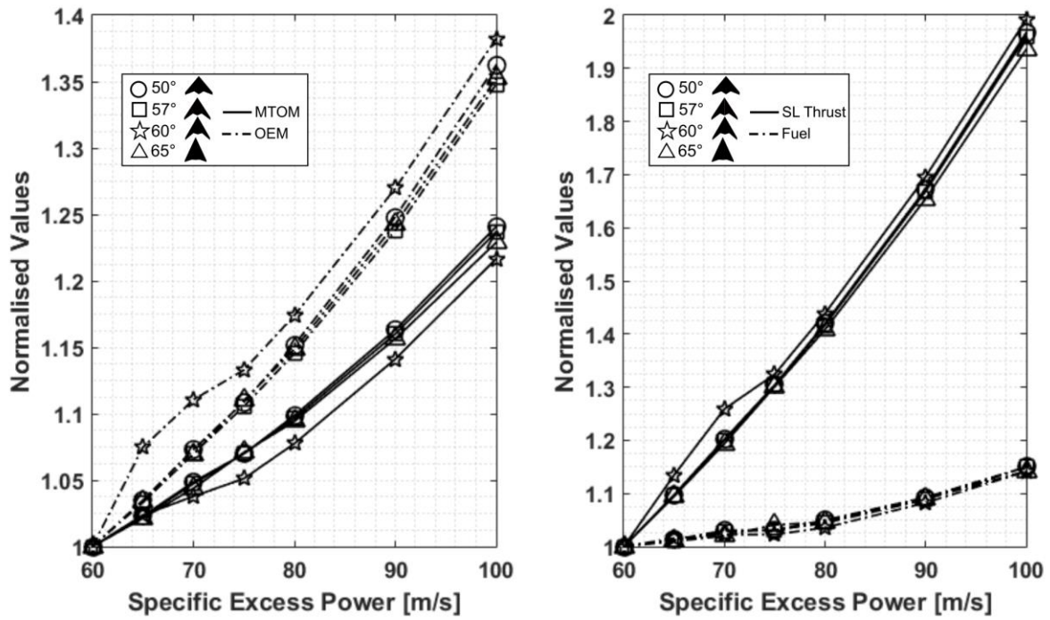
Figure 15 Effects of specific excess power on MTOM, OEM, fuel, and sea level thrust.
