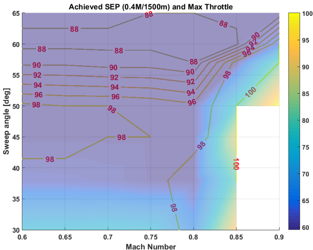
Figure 13 Specific excess power and maximum throttle setting for various cruise Mach numbers.
