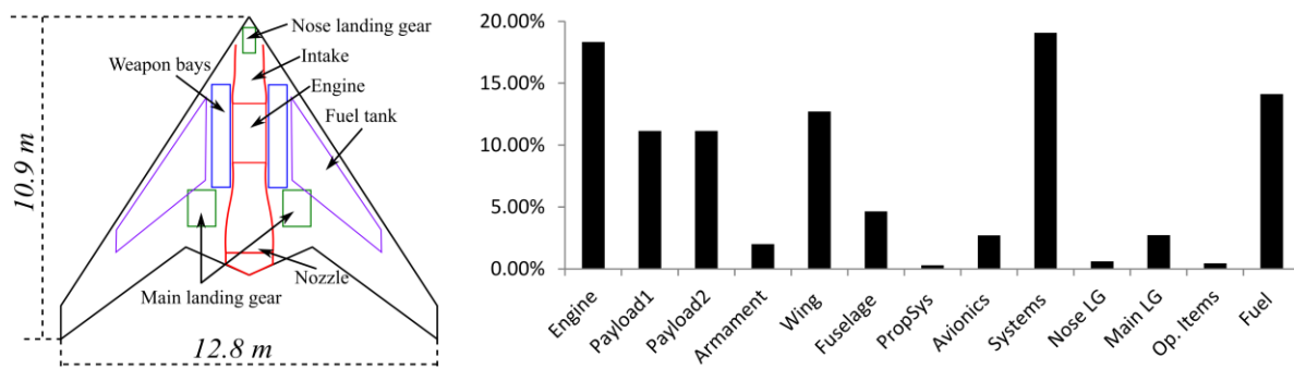
Figure 9 Baseline design top view and mass breakdown.
