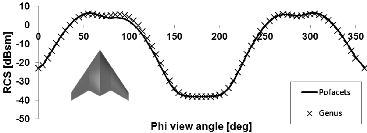
Figure 7 Monostatic RCS validation in GENUS.
